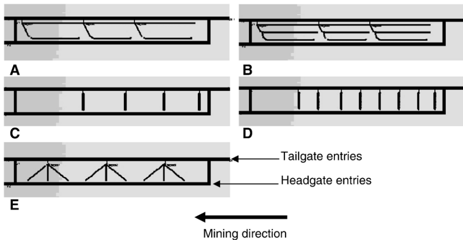
Fig. 4. Horizontal methane drainage borehole patterns modeled for degasification of the longwall panel. The entries represent a three-entry system with intervening coal pillars.
