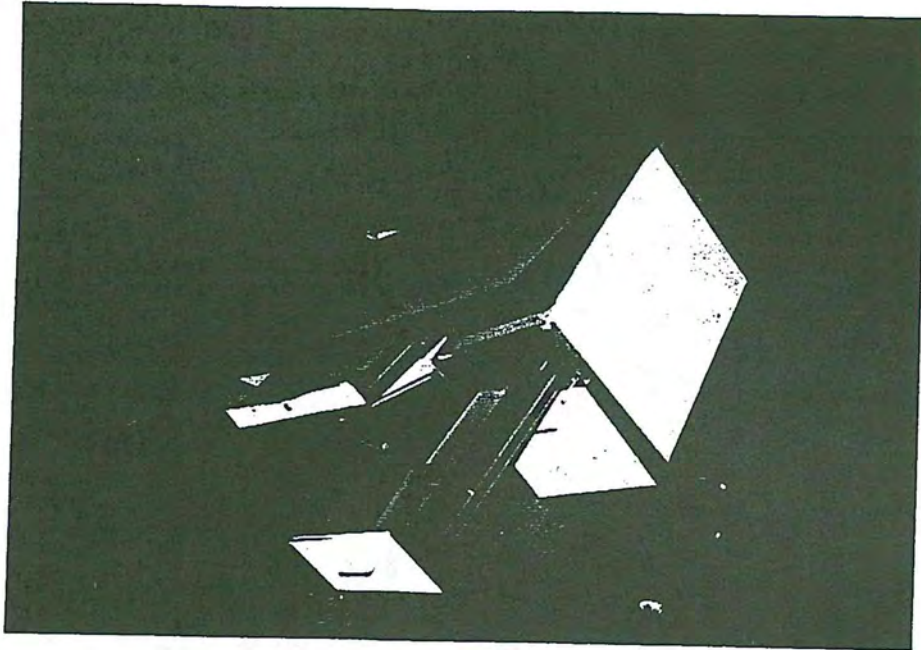
Figure 3-20. Minor damage to the desk located 200 ft down A-drift from the detonation of 20 lb of propylene oxide.
