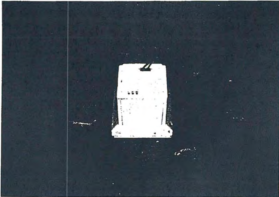
Figure 3-22. 200 ft down A-drift from the 20-1b propylene oxide detonation, the monitor was thrown to the floor but was not severely damaged.
