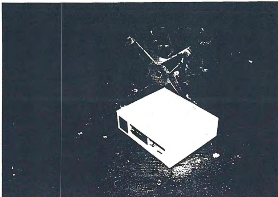
Figure 3-23. 200 ft down A-drift from the 20-1b propylene oxide detonation the computer was thrown to the floor but was not severely damaged.
