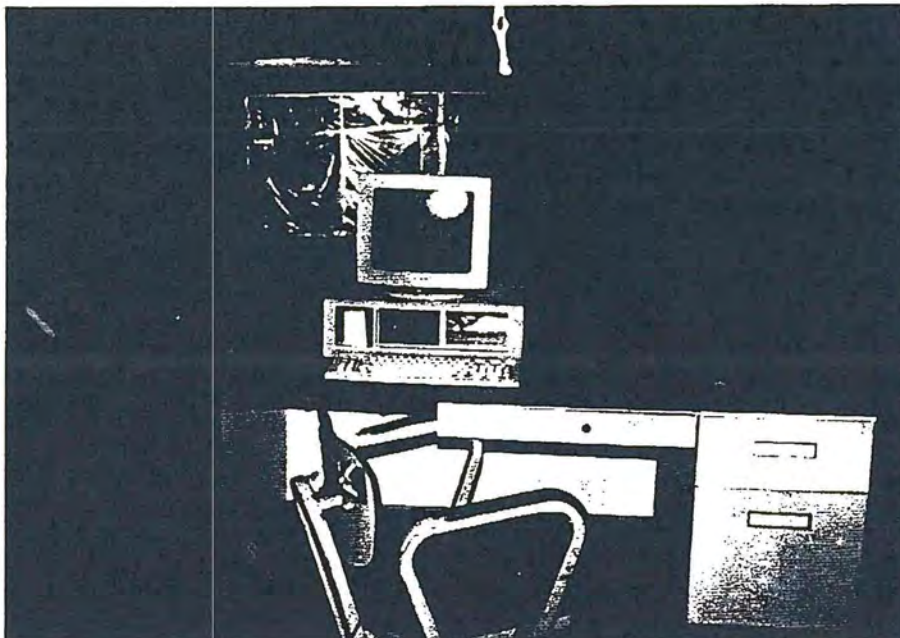
Figure 3-15. Desk, computer, monitor, and chair set up 60 ft down E-drift from the detonation of 20 lb of propylene oxide.
