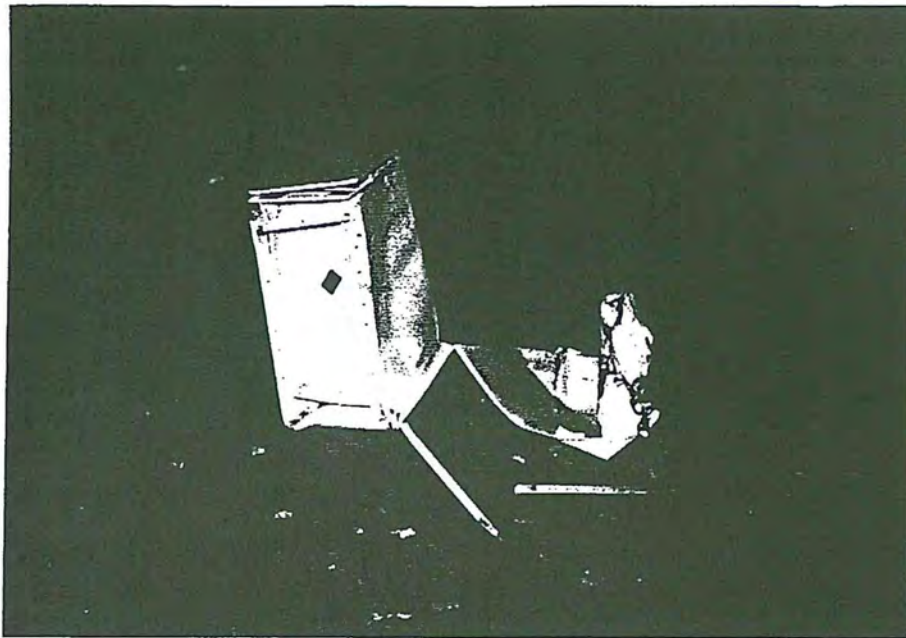
Figure 3-16. Damage to the desk located 100 ft down A-drift from the 20-lb propylene oxide detonation.
