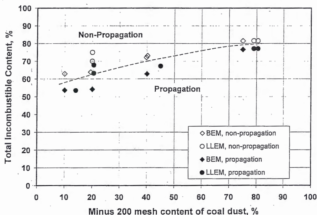
Fig. 2. Effect of particle size of coal dust on the explosibility.
