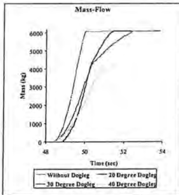
Figure 9. Effect of different configuration of Doglegs on mass-flow out of ore passes
