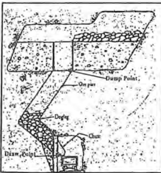
Fig. 1. Schematic of an ore pass system
