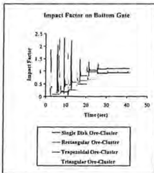
Figure 6. Impact factor on bottom gate for different shape ore-cluster
