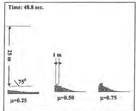
Figure 11. Snapshots of ore flow for different coefficient of frictions (not to scale)
