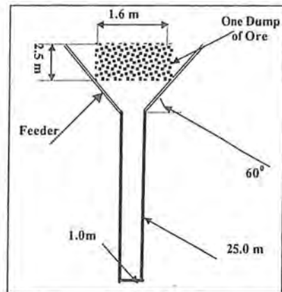
Fig. 5. Ore pass configuration (not to scale)
