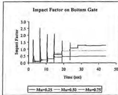
Figure 7. Effect of coefficient of friction on bottom gate impact factor
