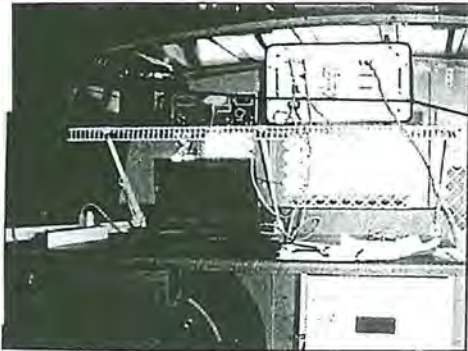
Figure 9.—Data acquisition system with electrode scanner (upper right), ABEM 300-C geoelectrical resistivity instrument (upper middle), auto battery (upper left), and laptop computer (lower middle).
