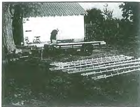
Figure 2.—Assembly of 1.3 cm (0.5 in) in diameter PVC pipe inserted into 2- by 4-in studs.
