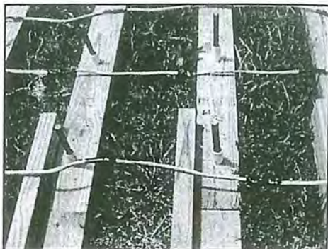
Figure 4.—Close-up of rebar electrodes sealed in plastic pipe and attached to electric cable.
