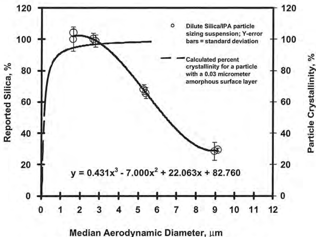
FIG. 2—Reported silica as determined by the MSHA P7 Method.
