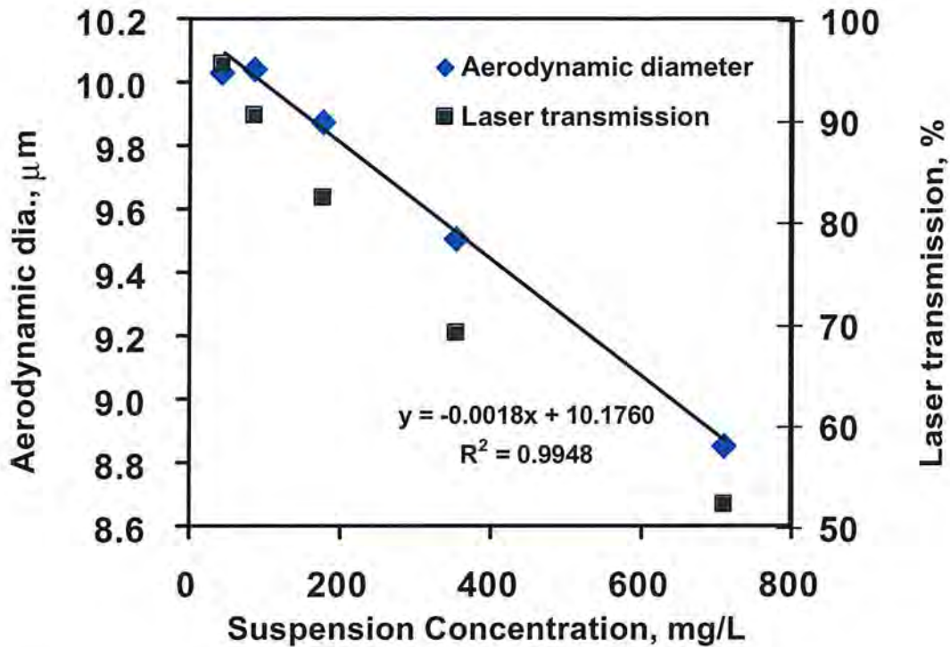
FIG. 1—Suspension concentration effect on the reported median aerodynamic sizes.
