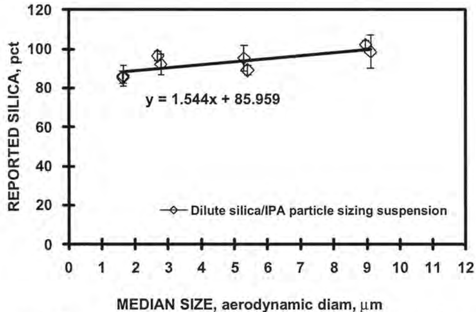
FIG. 3—NIOSH XRD Analytical Method 7500 results on same samples analyzed by MSHA P7 Method.
