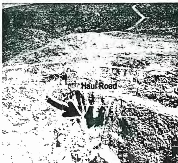
Figure 10. The overhang indicated by the arrow is a hazard to trucks traveling along the haul road because the drivers cannot see the portion of the slope that has failed below the road. The weight of the trucks on the partially failed material could cause the rest of the rock mass to fail.
