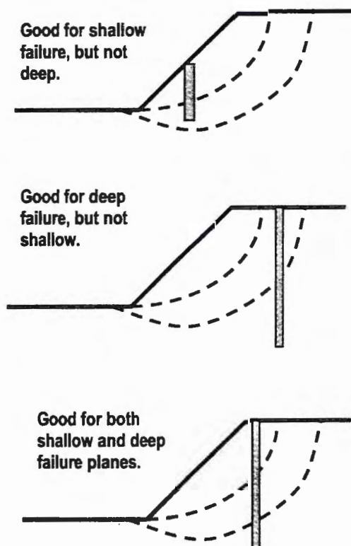
Figure 14. Proper inclinometer placement in a slope (adapted from Abramson et al., 1996)
