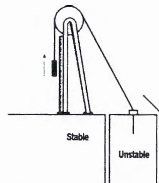
Figure 12. Wire-line extensometer.
