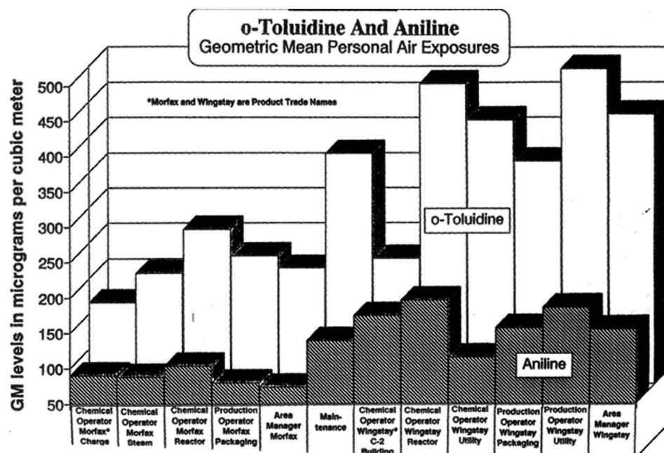
FIGURE 3 Average o-toluidine and aniline air concentrations by department in a chemical manufacturing plant, March 1990. Source: NIOSH Health Hazard Evaluation 11 (350 \mu\text{g}/\text{m}^3 corresponds to 0.08 ppm o-toluidine, 450 \mu\text{g}/\text{m}^3 corresponds to 0.10 ppm o-toluidine)
