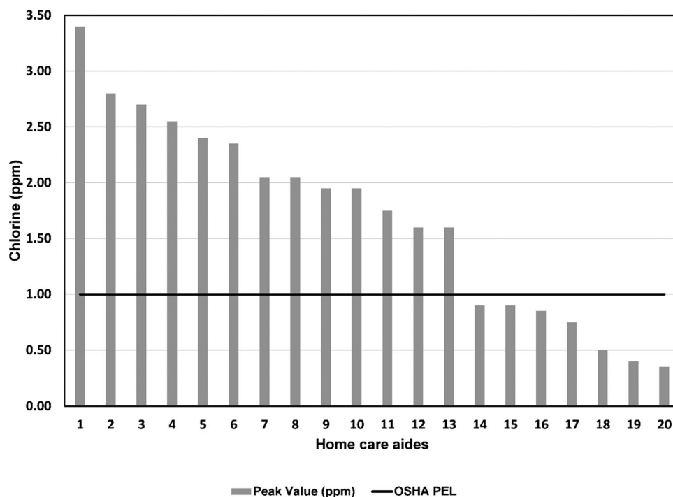
Figure 5. Peak chlorine ( \text{Cl}_2 ) gas concentrations generated by all study participants during bathroom cleaning with the bleach-based product compared to the US Occupational Safety and Health Administration Permissible Exposure Limit ceiling. OSHA PEL = US Occupational Safety and Health Administration Permissible Exposure Limit, 1.0 ppm ceiling limit.
