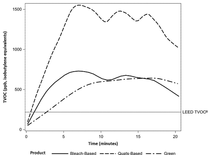
Figure 3. Total Volatile Organic Compounds (TVOC) concentration-time profiles A by product, all study participants' sessions combined using LOESS smoothing. A Each curve represents the smoothed TVOC concentration-time profile for all cleaning sessions using a specific product. The LOESS curve for the bleach-based product is based on 40 sessions; for the quats-based product, 40 sessions, and for the green product, 43 sessions (see text). B LEED TVOC = Leadership in Energy and Environmental Design criteria for indoor air TVOC concentration (500 \mu\text{g}/\text{m}^3 ) converted to a volume concentration in isobutylene equivalents (218 ppb) for comparison.
