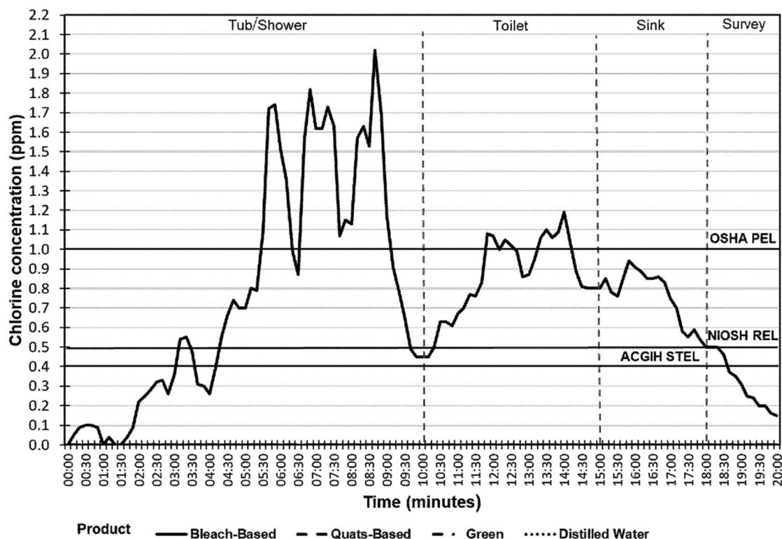
Figure 4. Chlorine ( \text{Cl}_2 ) gas concentration-time profile generated by one study participant performing bathroom cleaning using three products and distilled water. Note: Chlorine gas was monitored during the use of all products and distilled water; it was detected only during use of the bleach-based product. OSHA PEL = US Occupational Safety and Health Administration Permissible Exposure Limit, 1.0 ppm, ceiling. (NIOSH 2020). NIOSH REL = US National Institute for Occupational Safety and Health Recommended Exposure Limit, 0.5 ppm averaged over 15 min. (NIOSH 2020). ACGIH STEL = American Conference of Governmental Industrial Hygienists Short Term Exposure Limit, 0.4 ppm averaged over 15 min (ACGIH 2019).
