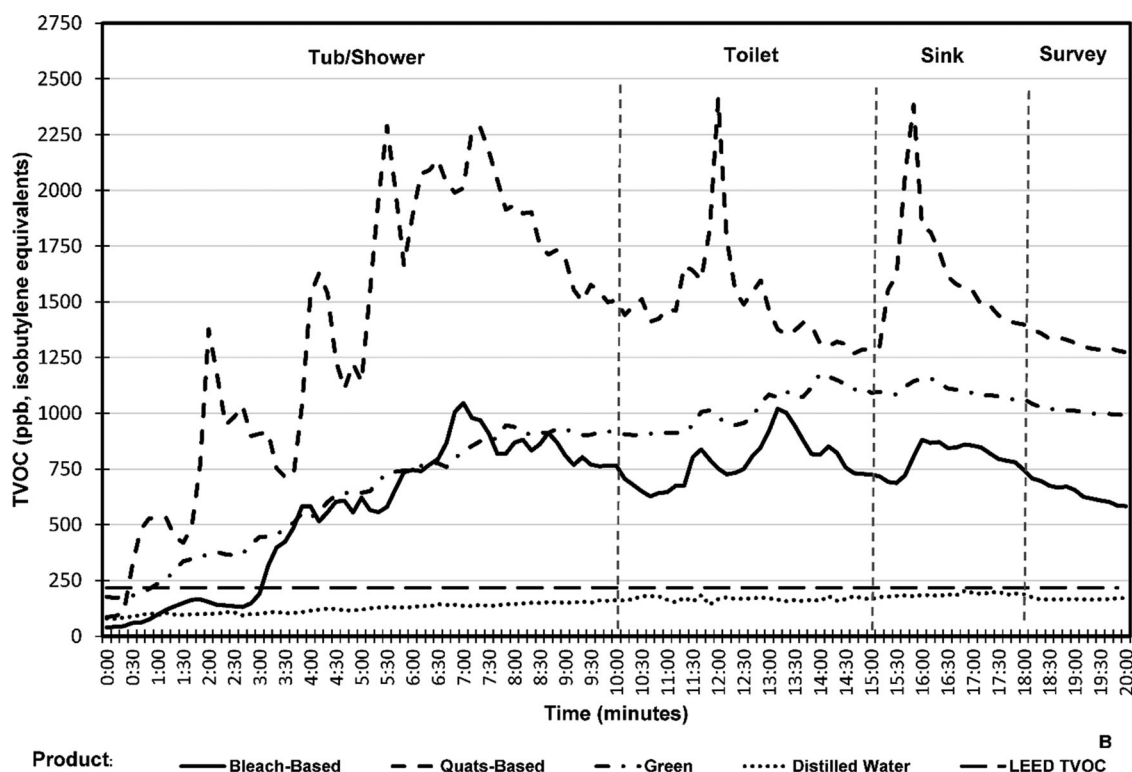
Figure 2. Total Volatile Organic Compounds (TVOC) concentration-time profiles A generated by one study participant performing bathroom cleaning using three products and distilled water. A TVOC concentration measurements: 10-sec averages over one 20-min cleaning session, converted to isobutylene equivalents. B LEED TVOC = Leadership in Energy and Environmental Design reference value for indoor air TVOC concentration ( 500 \mu\text{g}/\text{m}^3 ) converted to a volume concentration in isobutylene equivalents (218 ppb). (AIHA Construction and Toxicology Committees and Green Building Working Group 2017).
