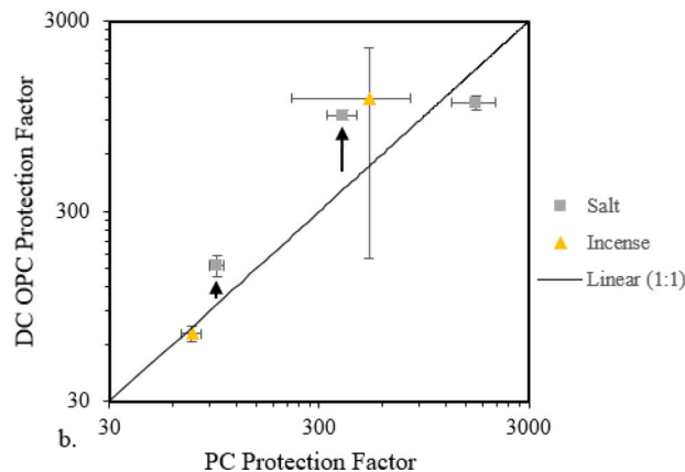
Figure 3. Arithmetic mean laboratory protection factor from the DC instruments compared to that from the PortaCount (indicated as PC) for (a) DC CPC and (b) DC OPC. The error bars represent the standard deviations for each of the three trials at each experimental level. The arrows represent the experimental levels where the null hypothesis is rejected. In these cases, the DC CPC underreported relative to the PC while the DC OPC generally over-reported relative to the PC.
