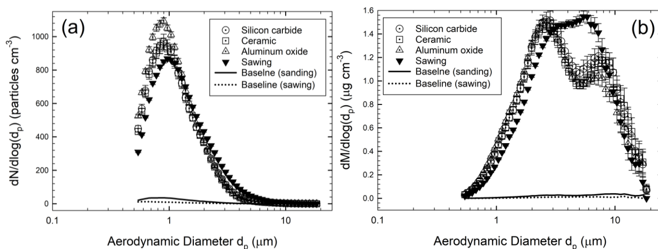
Fig. 3. (a) Number-based and (b) mass-based size distributions of the dust measured by APS from sawing and sanding (with sandpapers of ceramic, silicon carbide, and aluminum oxide) Corian ® .
