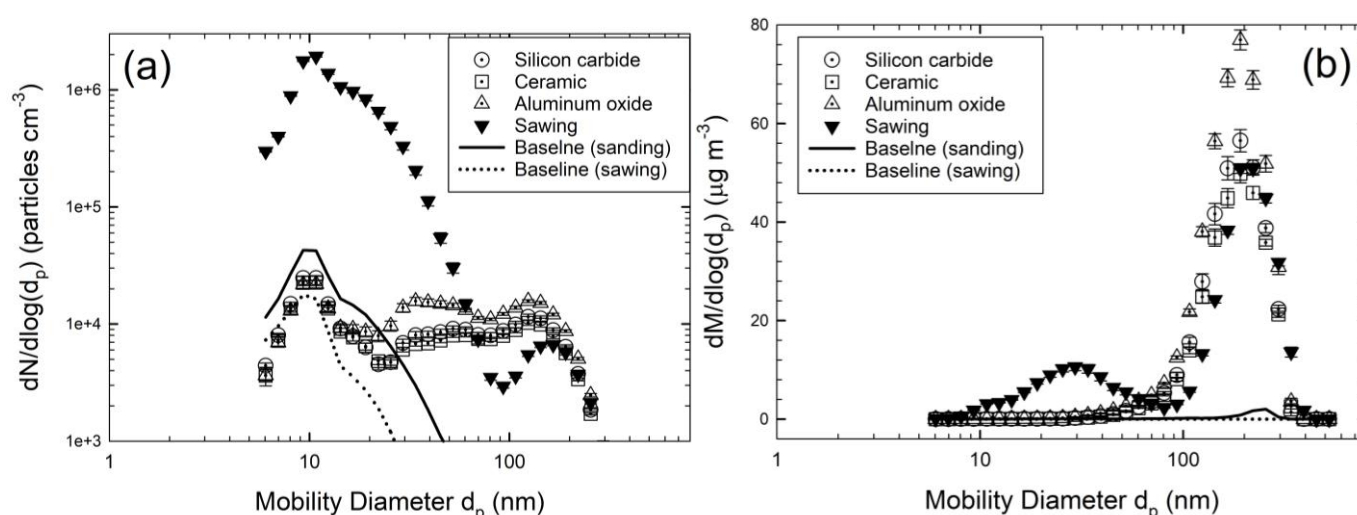
Fig. 2. (a) Number-based and (b) mass-based size distributions of the dust measured by FMPS from sawing and sanding (with sandpapers of ceramic, silicon carbide, and aluminum oxide) Corian®.
