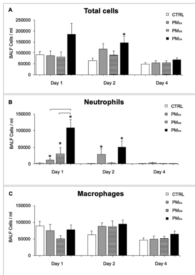
Fig. 1. Particulate matter (PM) extracts from California produced more inflammatory responses in bronchoalveolar lavage fluid (BALF) than those from China. Total cell (A), neutrophil (B), and macrophage (C) counts are shown for mice exposed to Milli-Q water vehicle control (CTRL) or particulate matter extracts from Taiyuan, Shanxi (PM SX ); Jinan, Shandong (PM SD ); or Sacramento, California (PM CA ), and sacrificed 1, 2, or 4 days post exposure. Data are presented as the mean \pm standard error of the mean. * indicates a significant ( p < 0.05 ) difference from controls. Brackets indicate significant ( p < 0.05 ) differences between PM treatment groups for the same day. N = 18/group (6/group/necropsy day).
