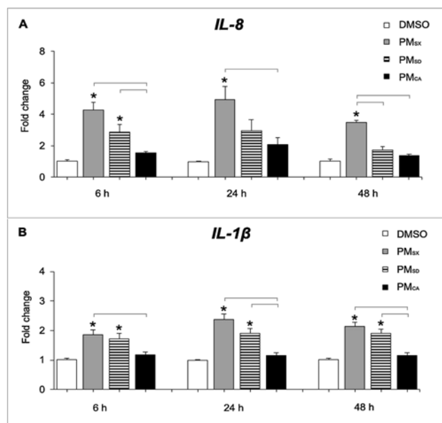
Fig. 7. PM SX significantly increased IL-8 and IL-1β mRNA levels in U937 macrophages following 6, 24, or 48 h of exposure. Graphs show results from qPCR analysis of cells treated with DMSO (control) or PM extracts from Taiyuan, Shanxi (PM SX ); Jinan, Shandong (PM SD ); or Sacramento, CA (PM CA ) for 6, 24, or 48 h. Gene expression is shown as a fold-change from expression of the housekeeping gene, ACTB (beta-actin). Data are shown as mean \pm SEM from experiments performed in triplicate. * indicates a significant difference ( p < 0.05 ) from control. Brackets indicate significant ( p < 0.05 ) differences between PM-treated groups.
