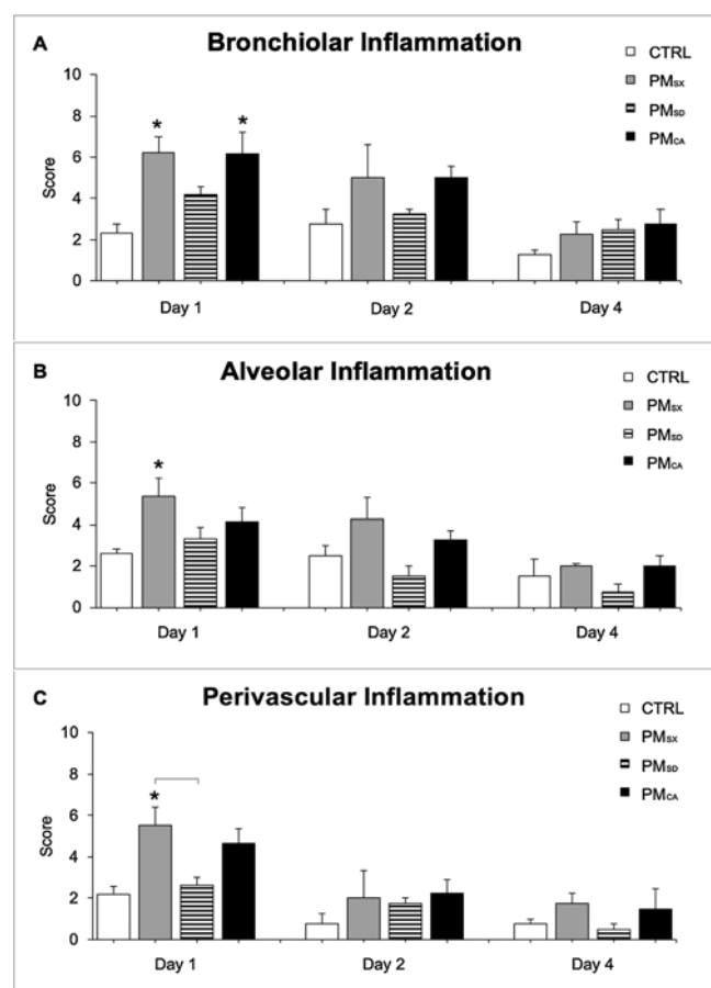
Fig. 2. Particulate matter extract samples from Shanxi, China (PM SX ) produced more histopathologic lung inflammation in mice. Graphs show semi-quantitative histopathology scores from the bronchiolar (A), alveolar (B), and perivascular (C) lung regions of mice exposed to Milli-Q water vehicle control (CTRL), or PM extracts from Taiyuan, Shanxi (PM SX ); Jinan, Shandong (PM SD ); or Sacramento, CA (PM CA ), and necropsied 1, 2, or 4 days thereafter. Data are mean \pm standard error of the mean. * indicates a significant ( p < 0.05 ) difference from controls. Brackets indicate significant ( p < 0.05 ) differences between PM treatment groups. N = 18 mice/PM exposed group (6 mice/group/necropsy day).
