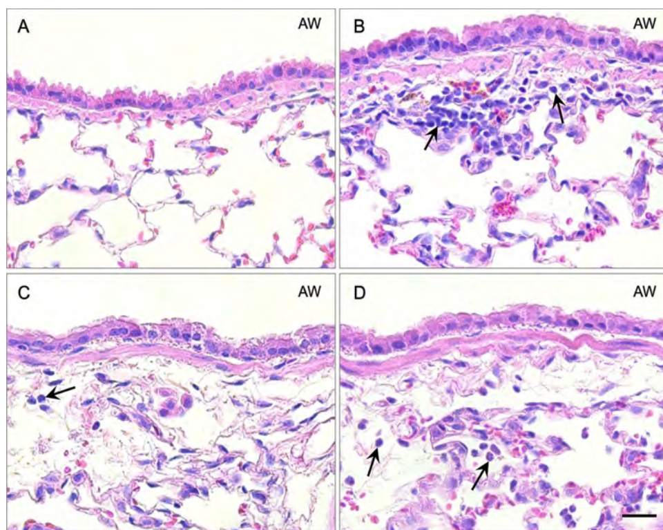
Fig. 3. Particulate matter (PM) extracts from China and California produced peribronchiolar inflammation in exposed mice. Panels are light micrographs of hematoxylin and eosin-stained mouse lung tissues collected one day after oropharyngeal aspiration of Milli-Q water (A) or PM extracts from Taiyuan, China (B); Jinan, China (C); or Sacramento, CA (D). Arrows pinpoint peribronchiolar inflammation. Scale bar is 20 \mu m. N = 18 mice/group (6 mice/group/necropsy day).
