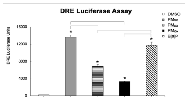
Fig. 5. Of the three PM extracts, PM SX induced the greatest dioxin-responsive element (DRE) luciferase reporter activity in HepG2 cells. This activity corresponded to aryl hydrocarbon receptor activation in cells incubated with DMSO (control); PM extracts from Taiyuan, Shanxi (PM SX ); Jinan, Shandong (PM SD ); or Sacramento, CA (PM CA ); or benzo(a)pyrene (B[a]P). Data are shown as mean \pm SEM from experiments performed in triplicate. * indicates a significant difference ( p < 0.05 ) from control. Brackets indicate significant ( p < 0.05 ) differences between PM-treated groups.
