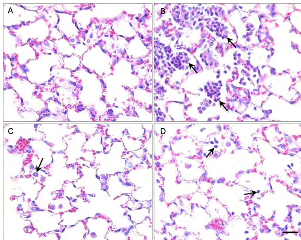
Fig. 4. Particulate matter (PM) extracts from China and California produced macrophagic alveolitis in exposed mice. Panels are light micrographs of hematoxylin and eosin-stained lung mouse tissues collected one day after oropharyngeal aspiration of Milli-Q water (vehicle control; A) or PM extracts from Taiyuan, China (B); Jinan, China (C); or Sacramento, CA (D). Arrows pinpoint alveolar inflammation. Scale bar is 20 \mu m. N = 18/group (6/group/necropsy day).
