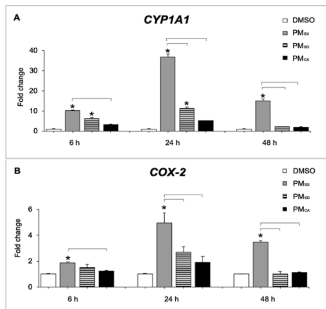
Fig. 6. PM SX significantly increased CYP1A1 and COX-2 mRNA levels in U937 macrophages following 6, 24, or 48 h of exposure. Graphs show results from qPCR analysis of cells treated with DMSO (control), PM extracts from Taiyuan, Shanxi (PM SX ); Jinan, Shandong (PM SD ); or Sacramento, CA (PM CA ) for 6, 24, or 48 h. Gene expression is shown as a fold-change from expression of the housekeeping gene, ACTB (beta-actin). Data are shown as mean \pm SEM from experiments performed in triplicate. * indicates a significant difference ( p < 0.05 ) from control. Brackets indicate significant ( p < 0.05 ) differences between PM-treated groups.
