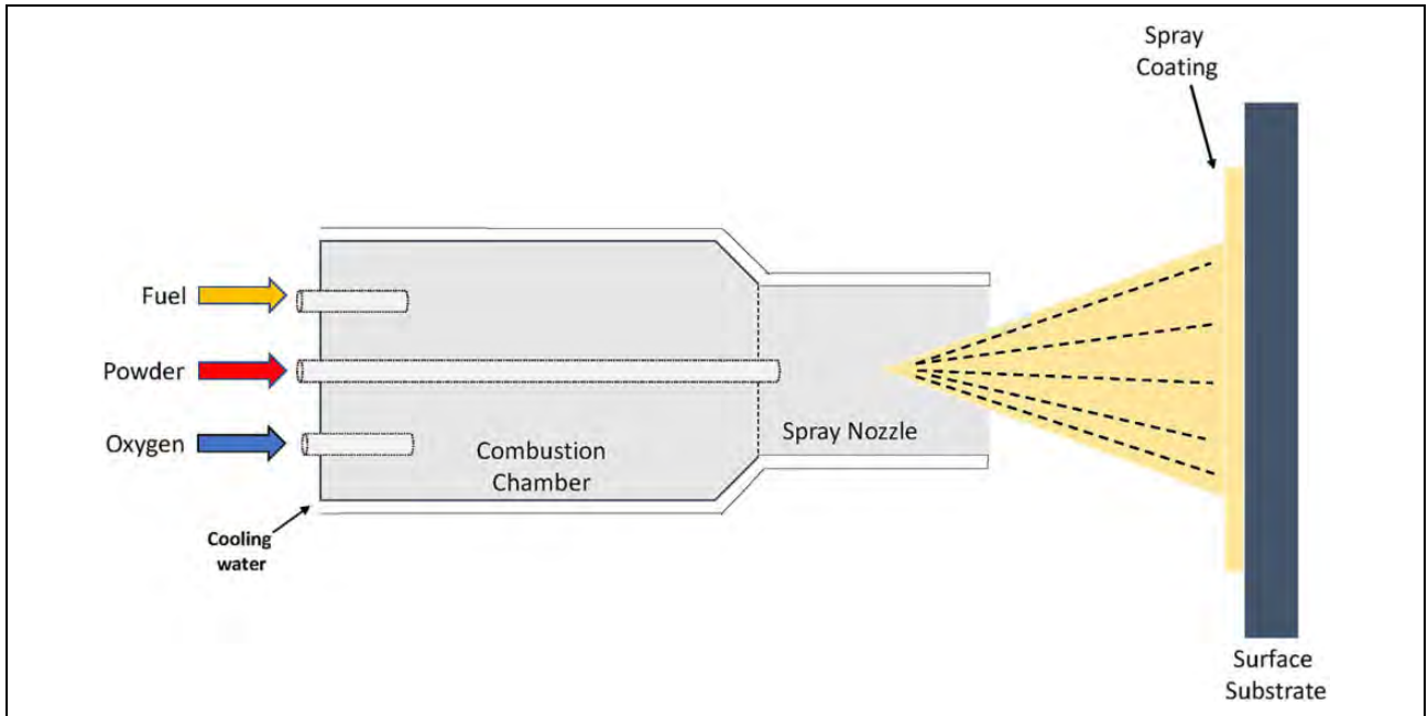
Figure 3. Thermal spray process: High-velocity oxy-fuel. Fuel gases are mixed with oxygen and burned in a chamber, resulting in expansion of the combustion products through the nozzle of a spray gun and significantly increasing in gas velocity. Powder is added to the nozzle, heated, and then accelerated with the expanding combustion products.
