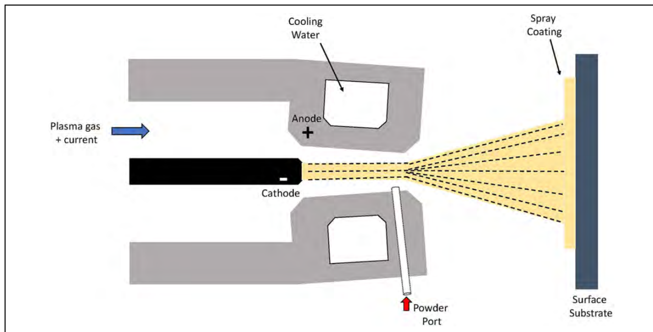
Figure 5. Thermal spray process: Plasma spray. A high-frequency arc is formed as superheated gas flows between an anode and a tungsten cathode, creating a high-pressure plasma plume. The spray coating material is introduced into the plasma as a powder where it is melted and propelled onto the surface to be coated.
