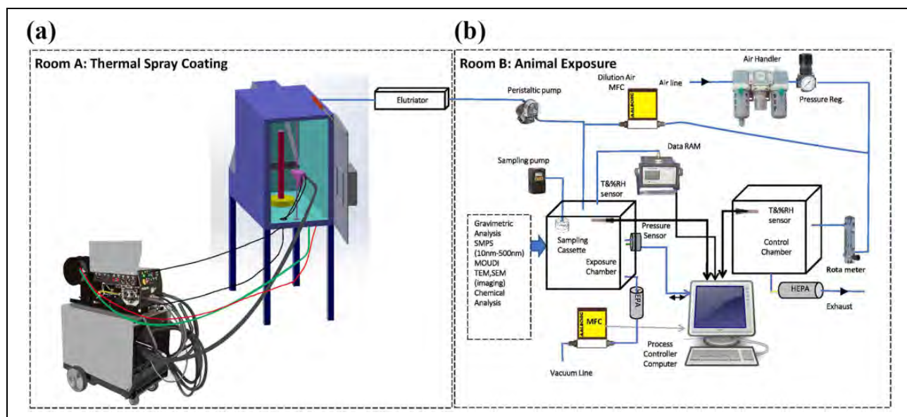
Figure 8. Schematic design of the electric arc wire thermal spray coating aerosol generation and exposure system. Thermal spray coating will be performed in one room (a), and the aerosols transferred to an exposure chamber in a separate room (b) divided by shaded glass doors (b). Data Ram: real-time aerosol monitor; MOUDI: micro-orifice uniform deposit impactor; SEM: scanning electron microscopy; TEM: transmission electron microscopy; T: temperature; RH: relative humidity; SMPS: scanning mobility particle sizer; MFC: mass flow controller.
