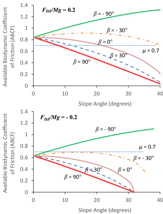
Fig. 5. The effect of the biodynamic normal force ( F_{DZ} ) on the ABCF as a function of the slope angle for several special cases ( \mu = 0.7 ; and \beta = -90^\circ, -30^\circ, 0^\circ, 30^\circ, 90^\circ ).
