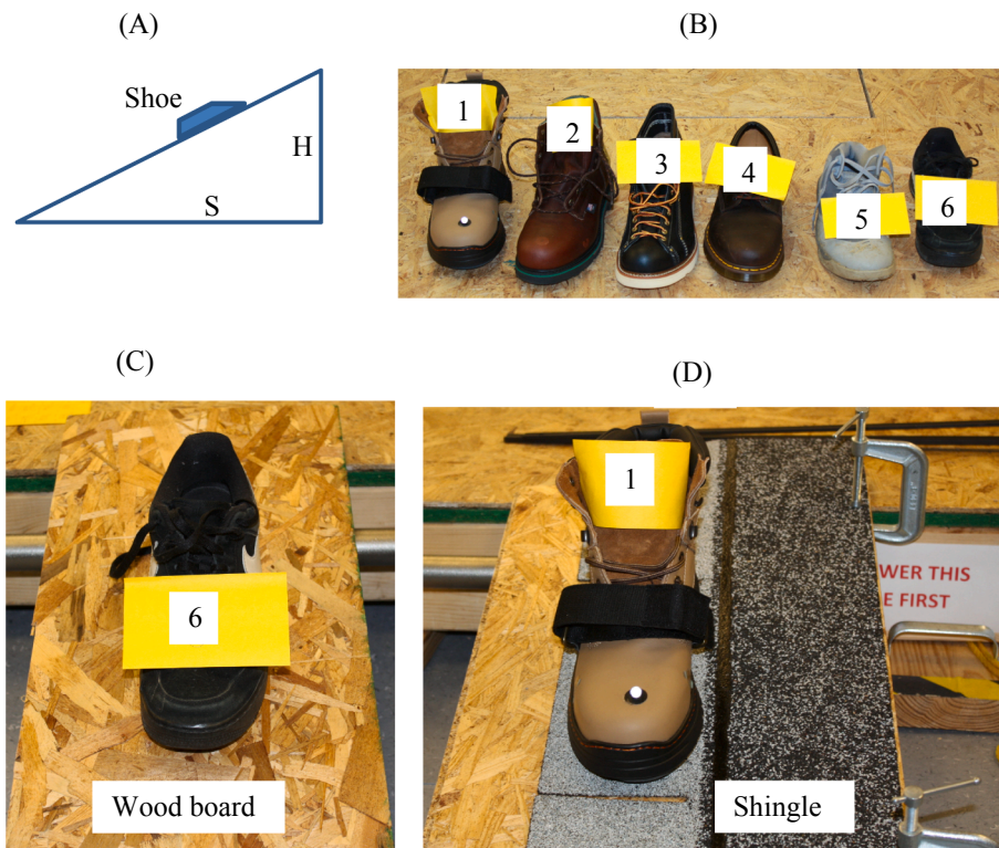
Fig. 2. The measurement of the coefficients of friction of six shoes on simulated roof surfaces: (A) Measurement principle; (B) Footwear tested for CF: 1–3 are roofer footwear and 4–6 are not considered roofer footwear; (C) Non-roofer footwear on oriented strand board (OSB); and (D) Roofer footwear on a standard asphalt shingle.
