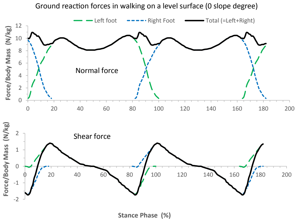
Fig. 3. The method for calculating the total ground reaction force in each direction: the measured left foot ground force reported by Redfern and DiPasquale (1997) + the right foot ground force that was assumed to be the same as that on the left foot except that its phase difference (with 18% overlap at the beginning and end of that for the left foot force); the forces were normalized with respect to body mass, the same as that in the original data.
