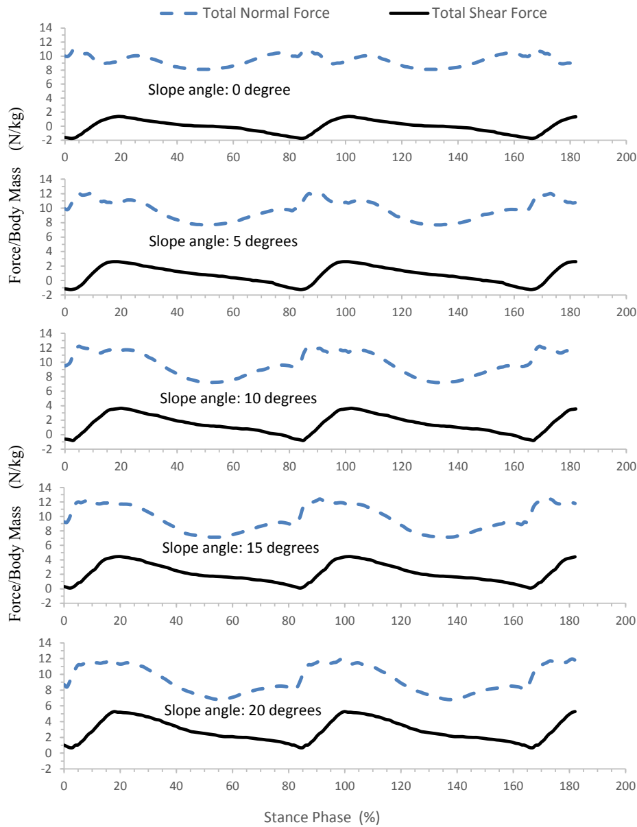
Fig. 6. The total ground forces for different slope angles (0°, 5°, 10°, 15°, and 20°), which were derived using the method illustrated in Fig. 3 from the experimental data reported by Redfern and DiPasquale (1997).
