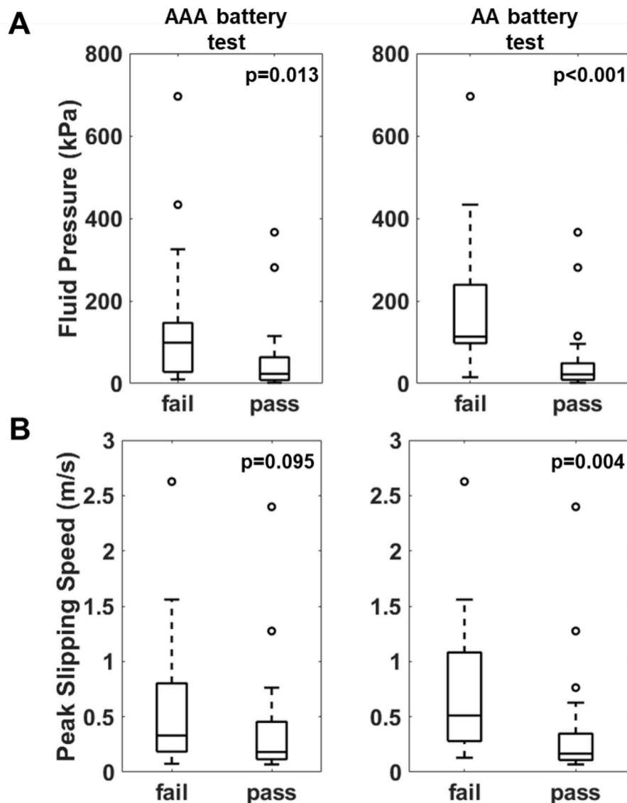
Fig. 3. Box plots of peak fluid pressure (A) and peak slipping speed (B) for fail/pass outcomes of the AAA battery test (left) and the AA battery test (right) from Experiment #3.
