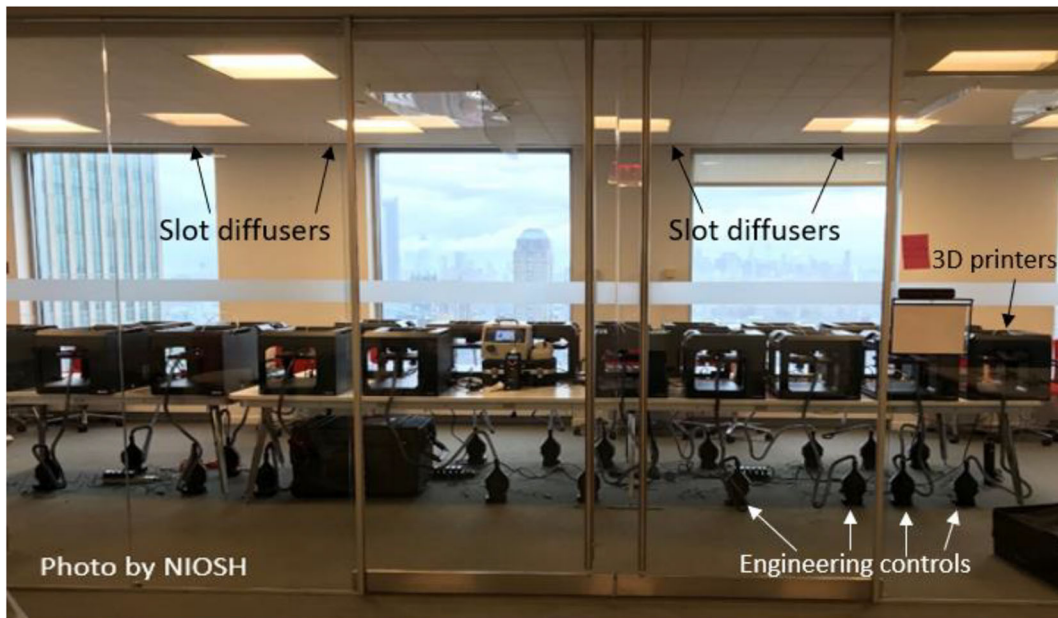
Fig. 2 Twenty MakerBot Replicator+3D printers with LEV engineering controls in a simulated makerspace (aka conference room). Photo by NIOSH
