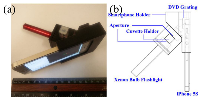
Fig. 1. (a) The assembled LeSSA, and (b) schematic structure of the LeSSA.
