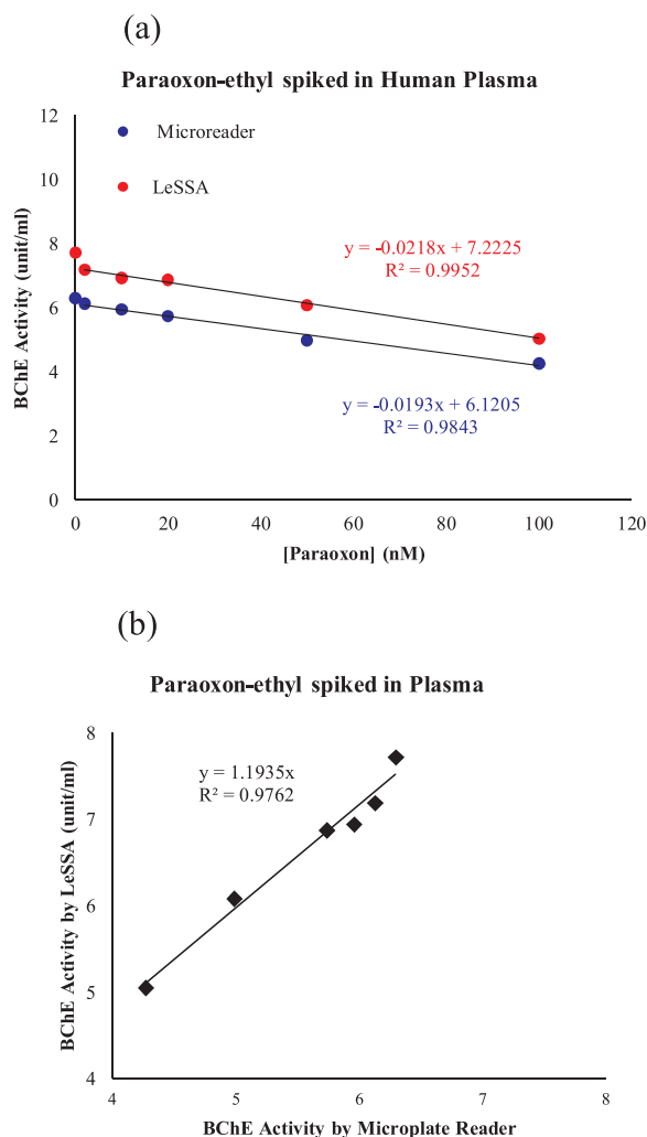
Fig. 5. (a) Linear regression for PChE activity in purchased human plasma related to Paraoxon-ethyl concentrations, and (b) linear correlation between PChE activity measured by the LeSSA and the microplate reader.
