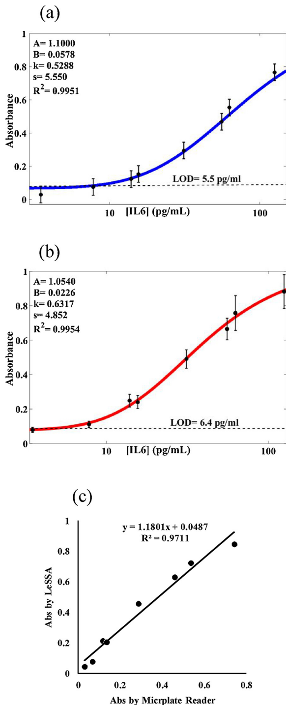
Fig. 3. Absorbance vs. IL-6 Concentration at 450 nm read by (a) the microplate reader, and (b) the LeSSA. (c) Linear correlation of the microplate reader and the LeSSA.
