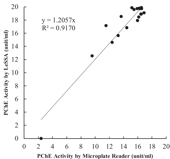
Fig. 6. The linear correlation between PChE activity measured in OP exposed plasma samples from agricultural workers, by the microplate reader and the LeSSA.
