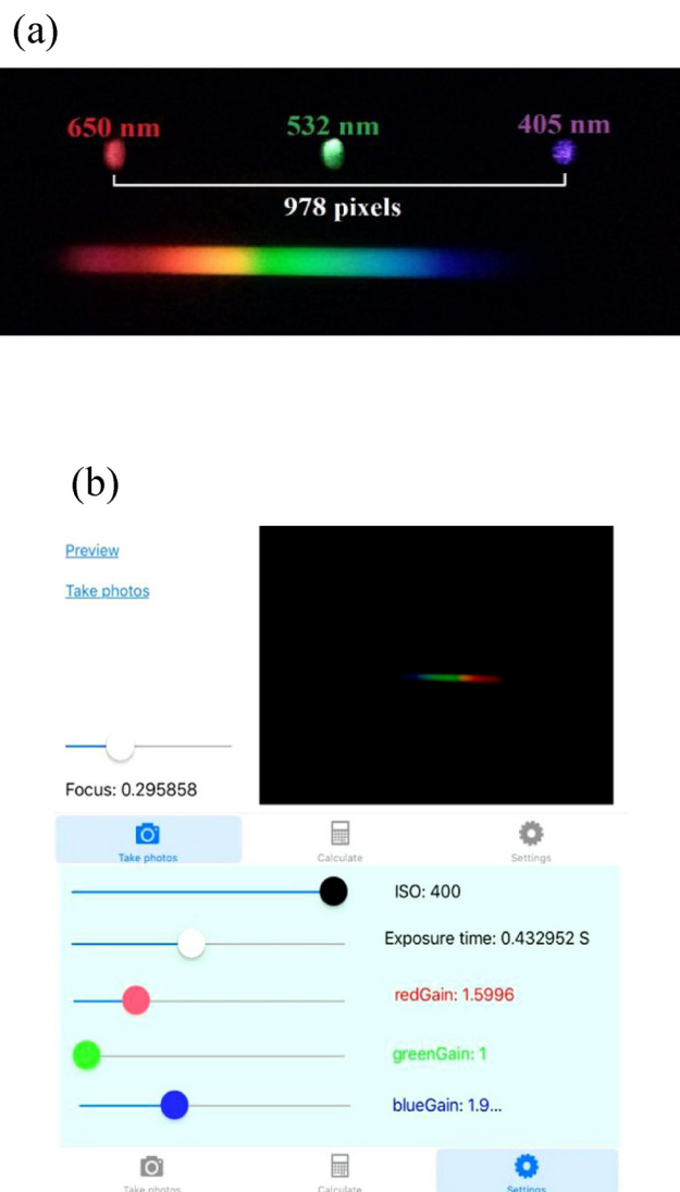
Fig. 2. (a) The mapping relationship in pixels and wavelength. (b) Self-developed photo-taking App to control the optical parameters (For interpretation of the references to colour in the text, the reader is referred to the web version of this article.).
