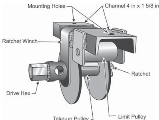
Figure 5. Ratchet assembly for hoisting EZ-Up Curtain Stopping.
