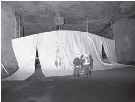
Figure 6. Raising the EZ-Up Curtain Stopping into position.
