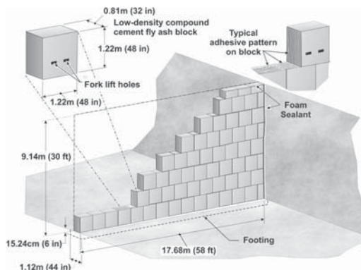
Figure 1. Schematic of Super Stopping.
