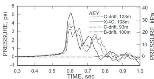
Figure 4. Pressure traces for the block stopping in X-4 during LLEM test #428.
