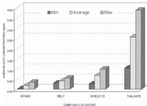
Figure 3. Range of dust concentrations measured at the stationary sampling locations.
