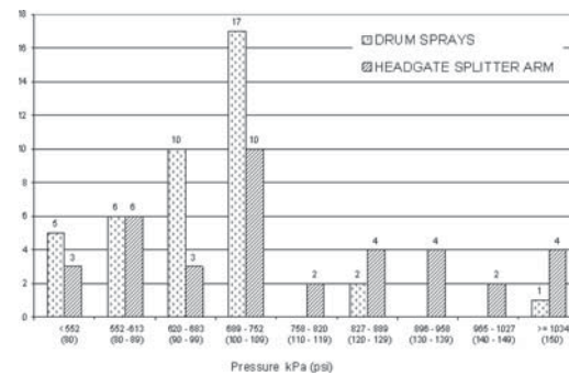
Figure 2. Pressure ranges for shearer drums sprays and splitter arm sprays.
