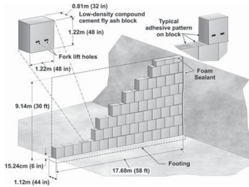
Figure 2. Schematic of super stopping.
