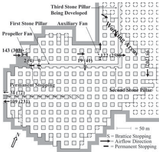
Figure 4. Ventilation airflows of new mine with long stone pillars. (Bold numbers are ventilation airflow volumes, \text{m}^3/\text{s} , ( \times 1000 cfm).
