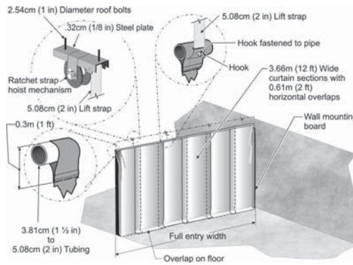
Figure 3. Schematic of EZ-Up stopping.
