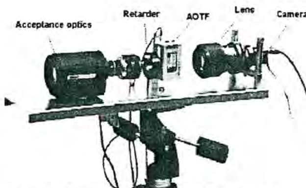
Figure 6. Carnegie-Mellon Research Institute's Spectro-polarimetric Imager.
