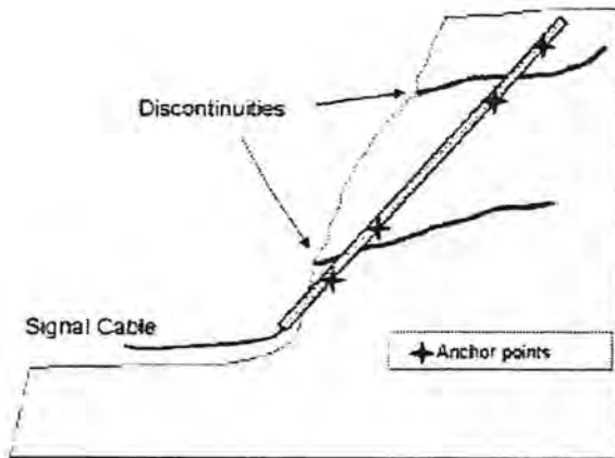
Figure 5. Multi-point borehole extensometer.
