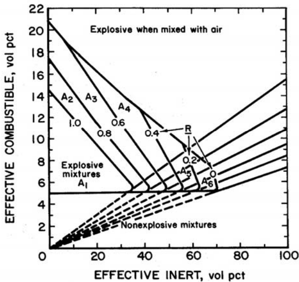
Figure 3. Explosibility diagram
