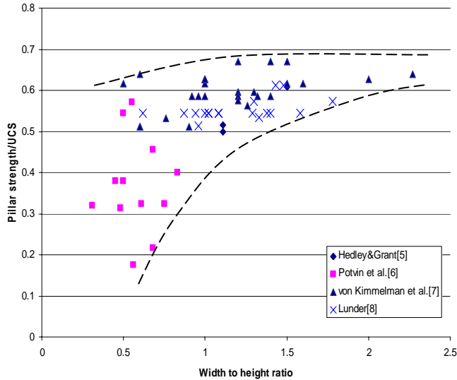
Figure 1. Pillar stability graph showing published case histories of failed pillars from hard rock metal mines
