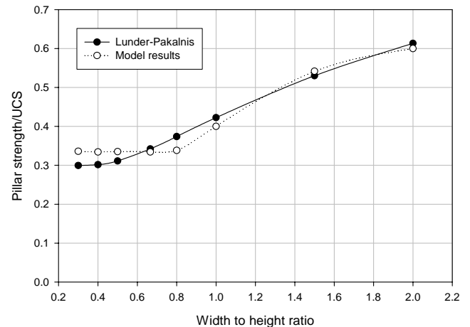
Figure 5. Results of model calibration against the Lunder-Pakalnis [9] empirically derived pillar strength equation.
