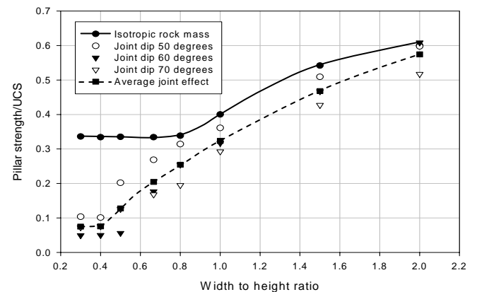
Figure 8. Numerical model results of pillar strength versus width to height ratio, showing the effect of discontinuities inclined at 50 to 70 degrees on pillar strength.
