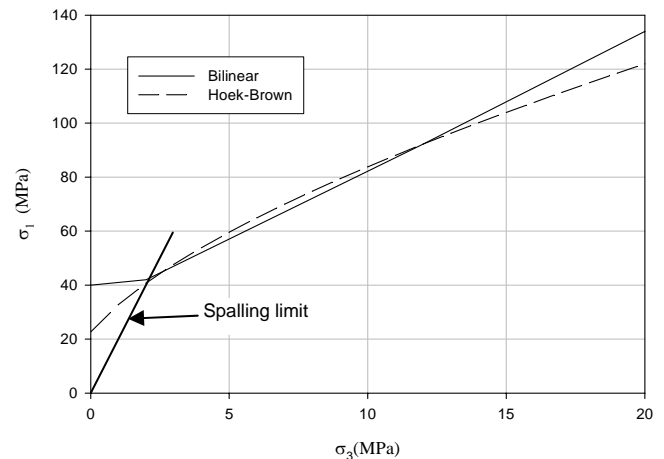
Figure 3. Bilinear and Hoek-Brown[13] rock strength plots for a Rock Mass Rating of 70.0
