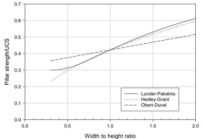
Figure 2. Comparison of pillar strength equations.
