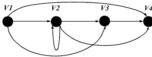
Fig. 3. A nonlinear system having five paths.
