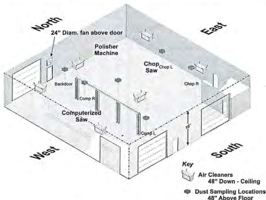
FIG 4 - Air cleaner units and dust sampling locations.
