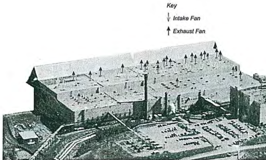
FIG 3 - Ventilation setup #3.
