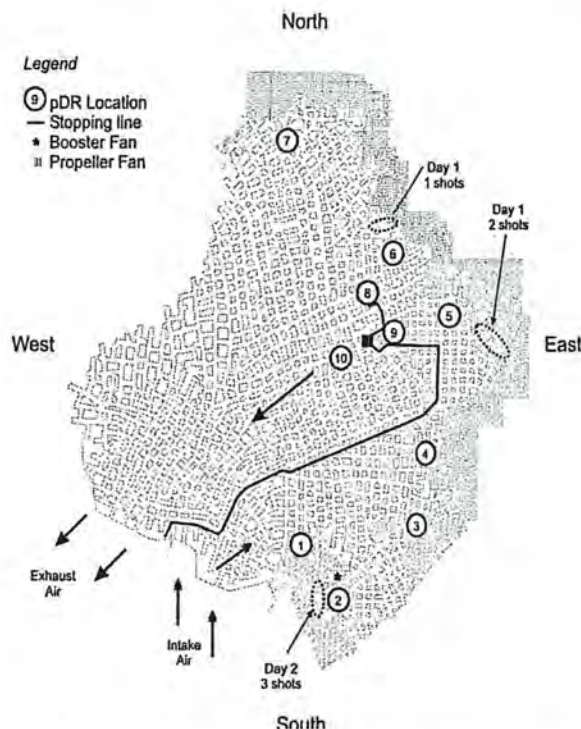
FIG 6 - Mine workings for case study, showing location of dust monitors, curtain line, and fans.
