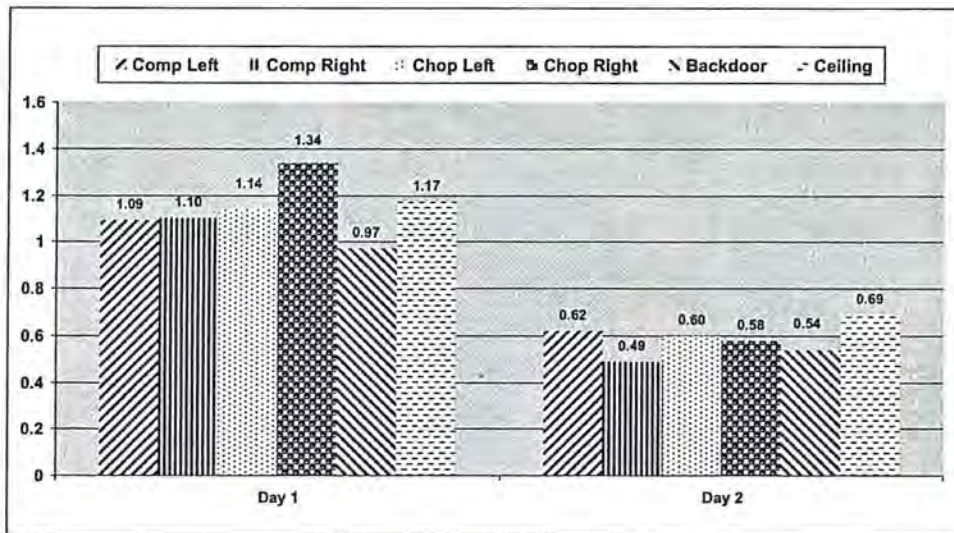
FIG 5 - Respirable dust concentrations in mg/m^3 for filters that had been in operation for three to four months (day one) and new filters (day two) on six air cleaning units.
