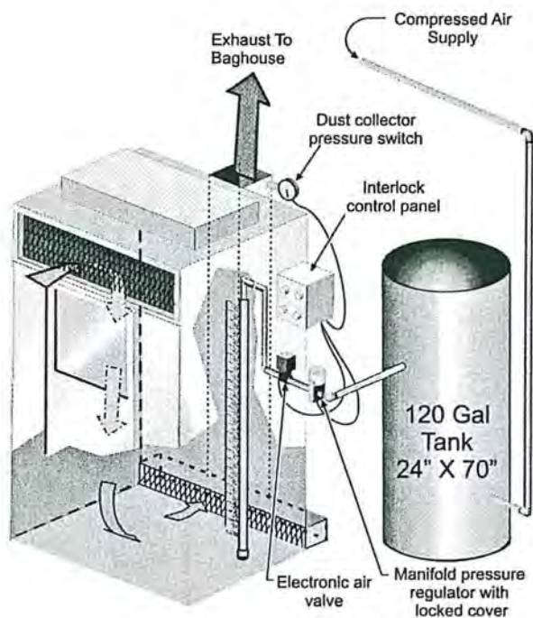
FIG 8 - Clothes cleaning technique design.
