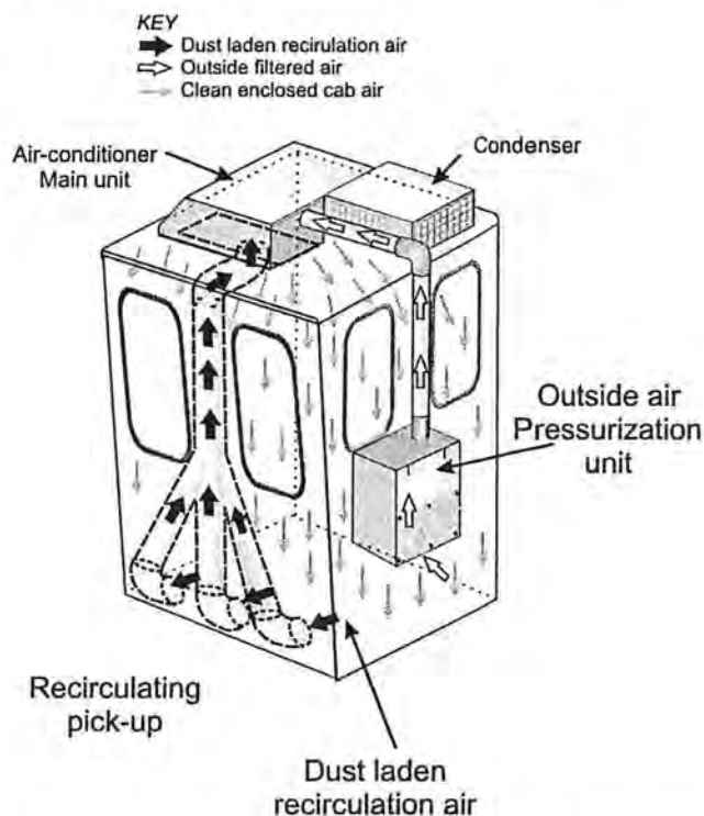
FIG 7 - Schematic for effective filtration and pressurisation system.
