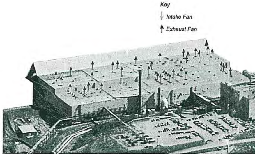
FIG 1 - Baseline or normal ventilation setup.
