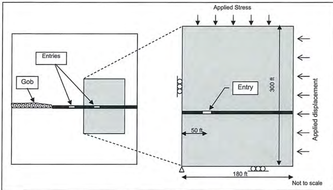
Figure 6. FLAC model geometry and boundary conditions.
