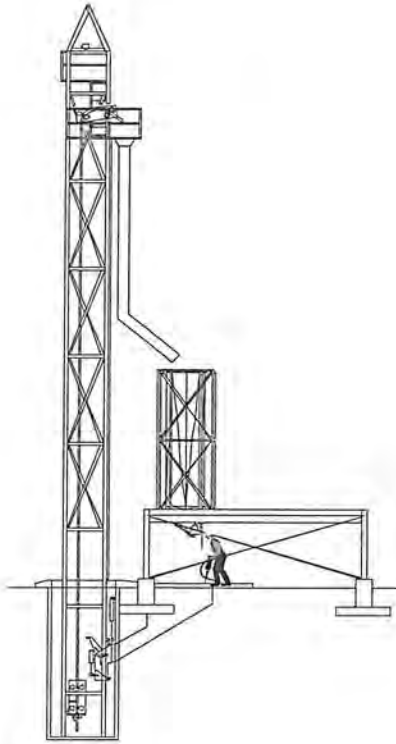
Figure 1. Reduced-scale hoist and ore pass test facility.
