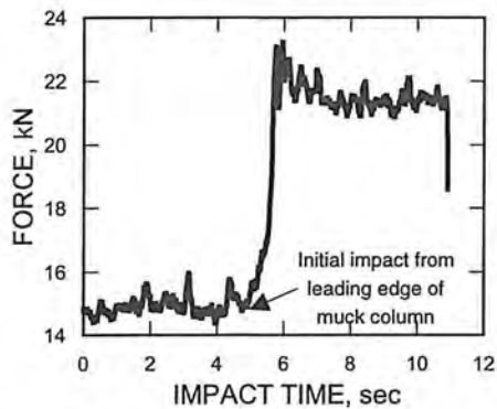
Figure 4. Impact forces on chute support structure.
