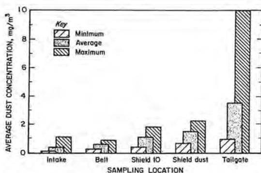
Figure 3. Range of dust concentrations measured at stationary sampling locations and for shield advance.
