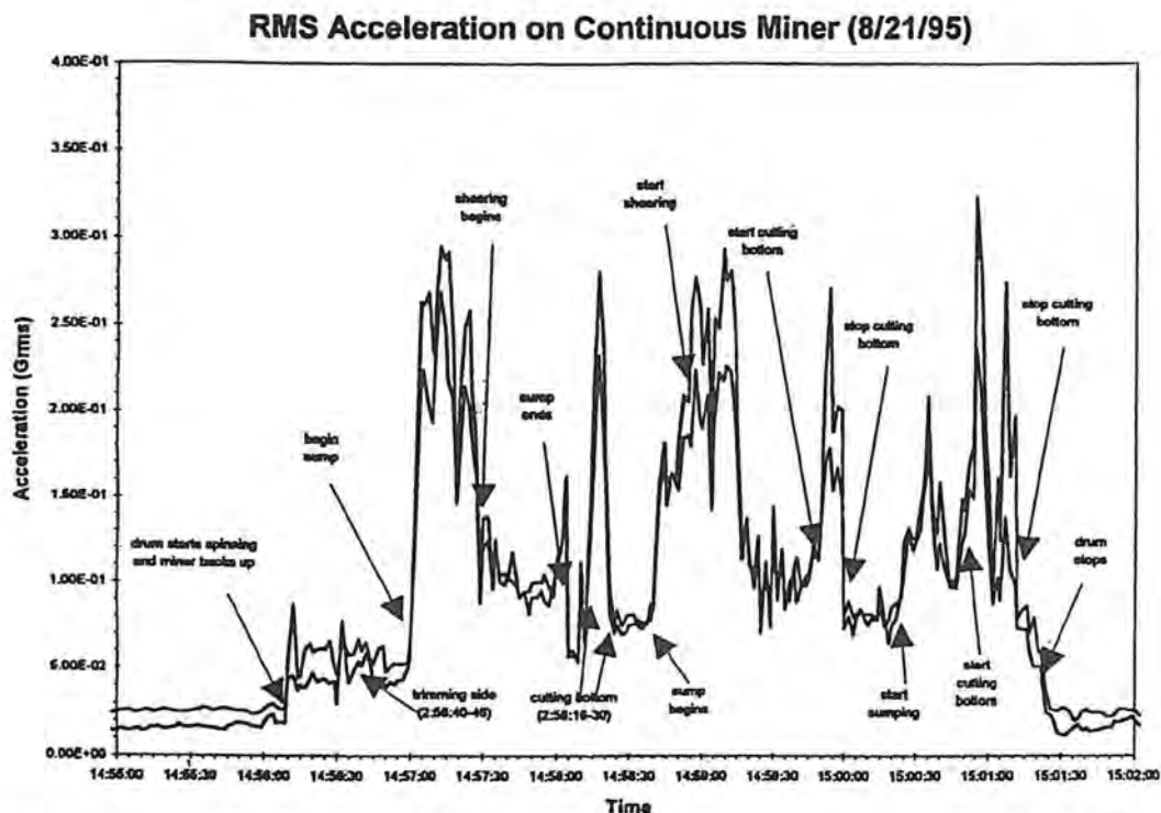
Figure 5. Vibration measured at the MMCRDM on 21 August 1995.
