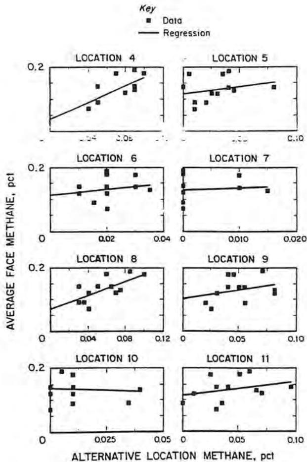
Figure 5. Comparison of methane concentrations at face and outby locations.
