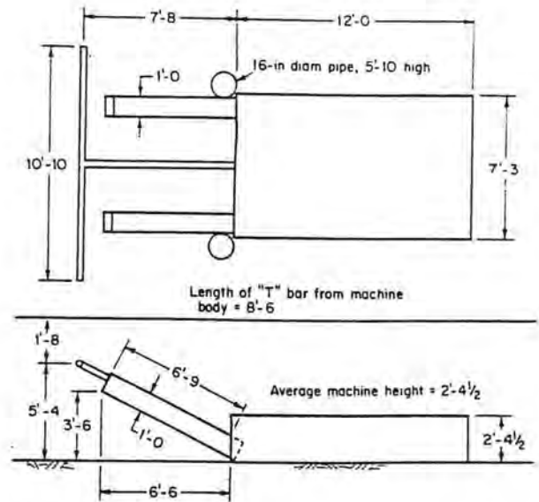
Figure 2. Model roof bolting machine.
