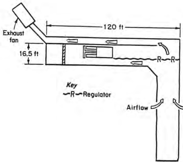
Figure 1. Methane test gallery.
