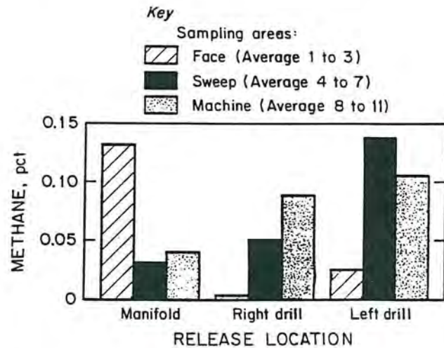
Figure 4. Effects of release location on concentration.
