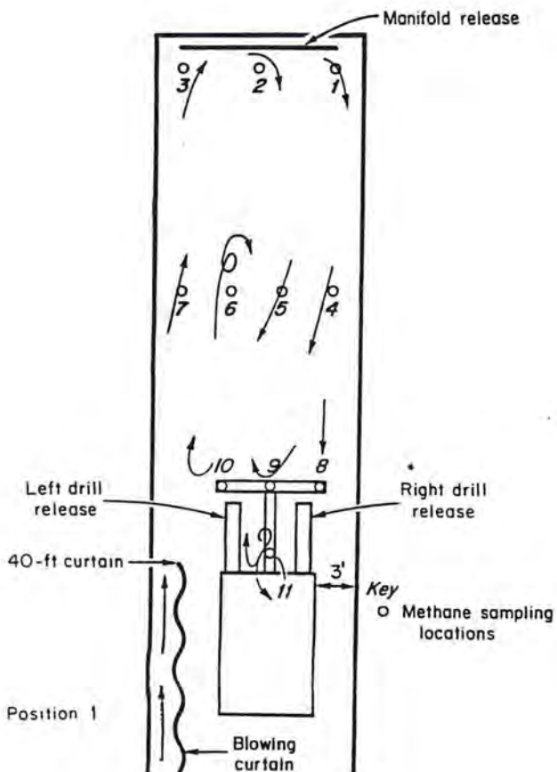
Figure 6. Face airflow patterns
