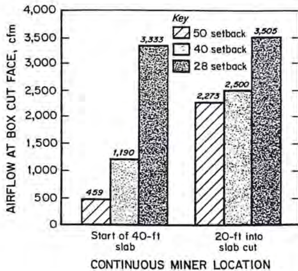
Figure 12 - Brattice setback effect (10,000 cfm intake/scrubber flow and 120 psi water pressure).
