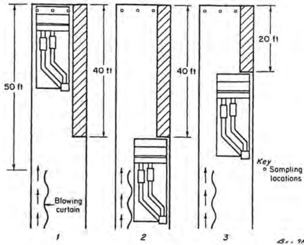
Figure 3 - First test series: continuous miner locations with 50-ft brattice setback distance
