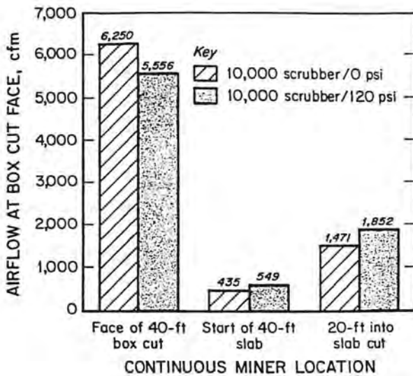
Figure 10 - Effects of water sprays (10,000 cfm intake).
