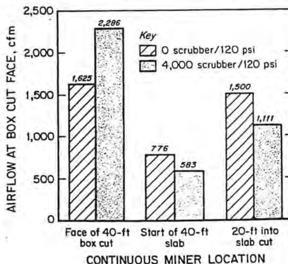
Figure 9 - Effects of scrubber flow (4,000 cfm intake).
