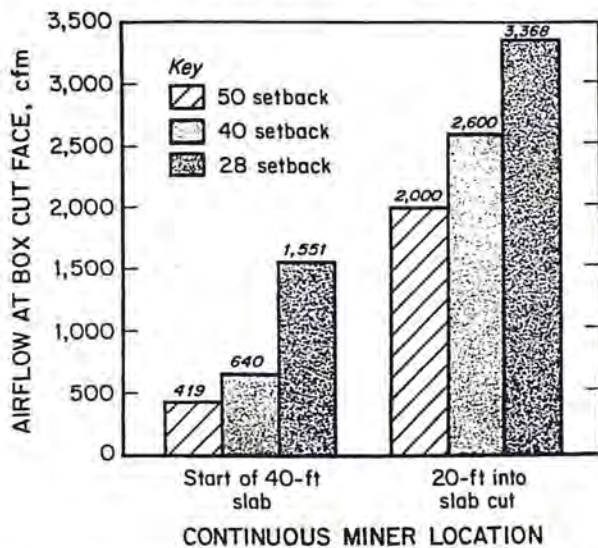
Figure 13 - Brattice setback effect (4,000 cfm intake/scrubber flow and 120 psi water pressure).
