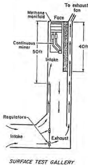
Figure 1 - Full-scale test gallery
