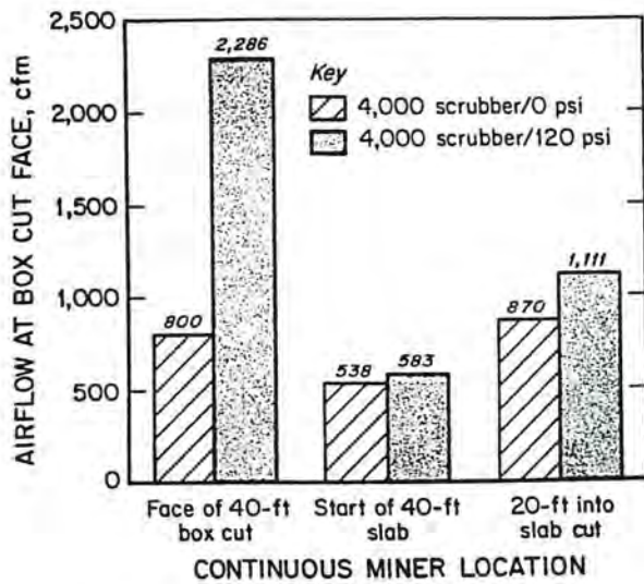
Figure 11 - Effects of water sprays (4,000 cfm intake).
