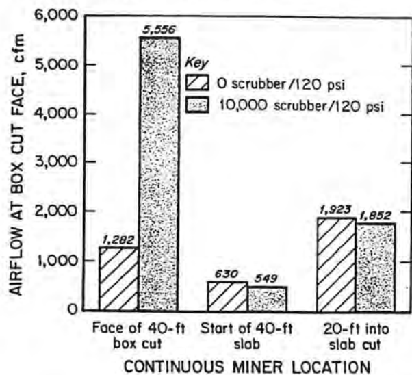
Figure 8 - Effects of scrubber flow (10,000 cfm intake).
