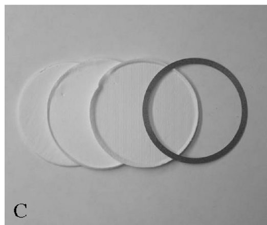
FIGURE 1. SKC DPM cassette: (A) The main casing used for both Design I and Design II. (B) Design I (manufactured before August 2002) and (C) Design II (instead of aluminum shield, a metal gasket followed by two quartz filters and a backing pad are used in this design)
