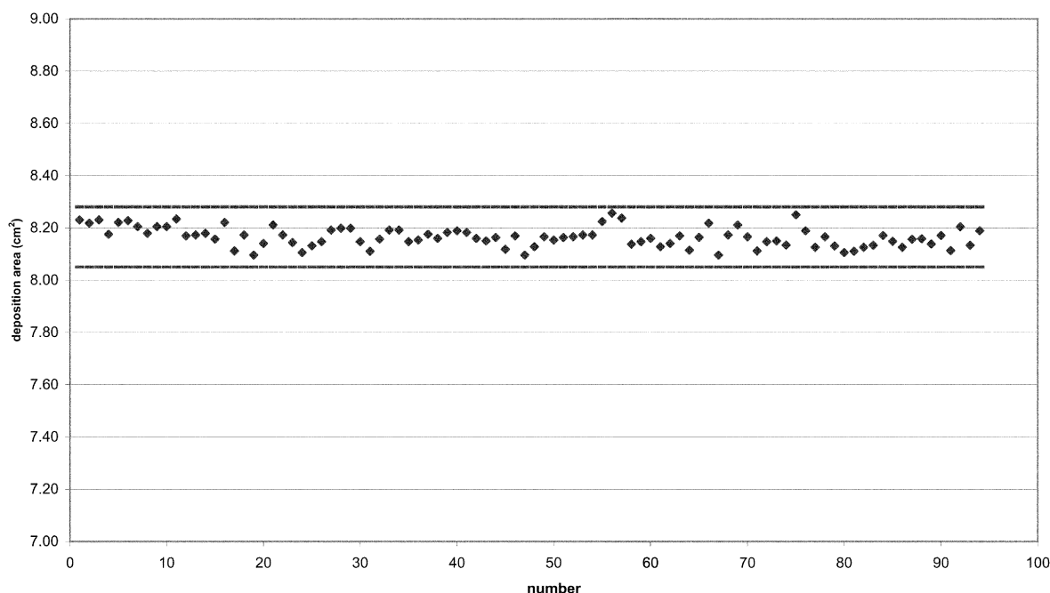
FIGURE 6. Ninety-four deposit areas of filters from Design II SKC DPM cassette (field and laboratory samples). The dotted lines are the upper and lower control limits.
