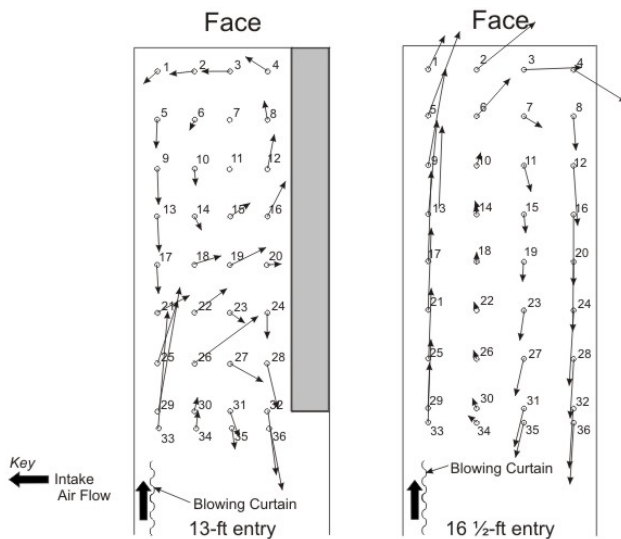
Figure 7. Flow diagrams for 35-ft setback.
