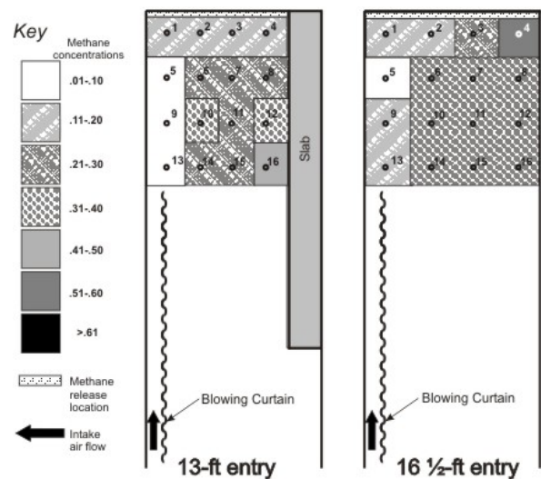
Figure 8. Methane profile for 15-ft setback, 10,000 cfm intake.
