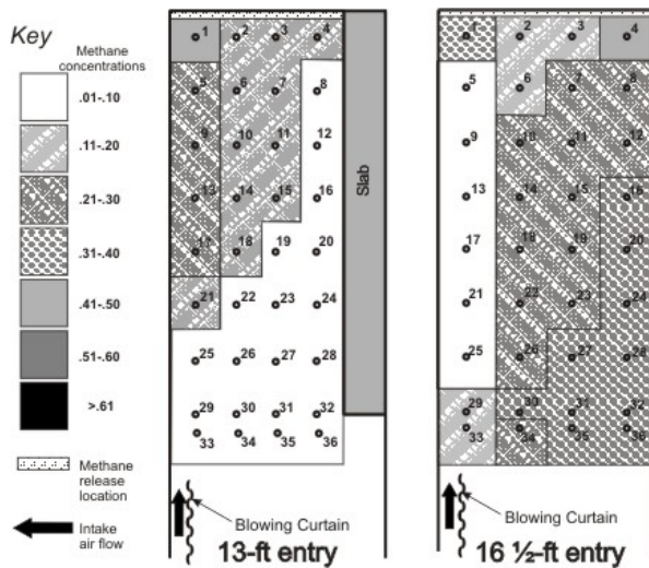
Figure 10. Methane distribution for 35-ft setback, 10,000 cfm intake.
