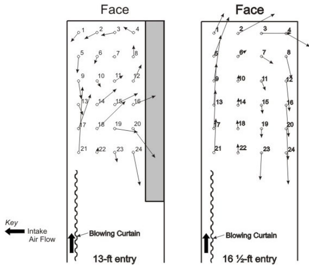
Figure 6. Flow diagrams for 25-ft setback.
