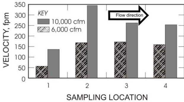
Figure 13. Twenty-five ft curtain setback, 16 ½-ft-wide entry.
