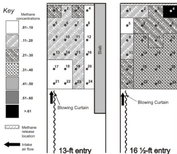
Figure 9. Methane distribution for 25-ft setback, 10,000 cfm intake.
