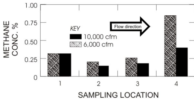
Figure 19. Methane concentration, 35-ft curtain setback, 16 ½-ft entry.
