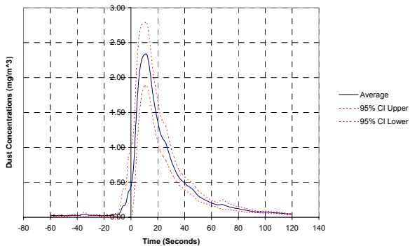
Figure 3. Average instantaneous respirable dust concentrations for Station B of the Coal Preparation Plant study.
