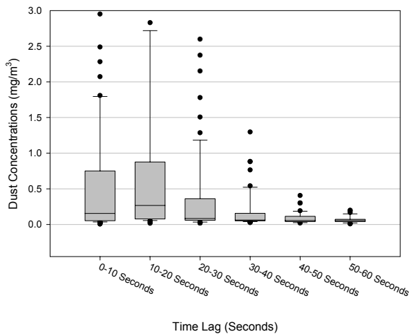
Figure 11. Instantaneous respirable dust concentrations from 0.0 - 3.0 mg/m 3 with time lag for Station B of the Stone Quarry Study.
