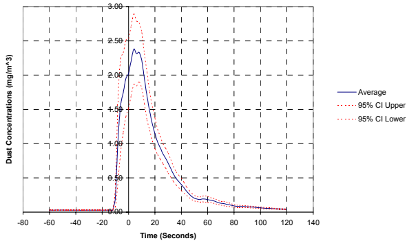
Figure 2. Average instantaneous respirable dust concentrations for Station A of the Coal Preparation Plant study.
