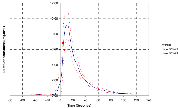
Figure 7. Estimated average instantaneous thoracic dust concentrations for Station B of the Coal Preparation Plant study.
