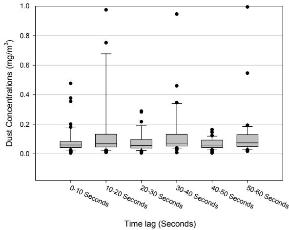
Figure 10. Instantaneous respirable dust concentrations from 0.0 - 1.0 mg/m 3 with time lag for Station A of the Stone Quarry Study.
