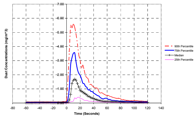
Figure 5. Percentile graph of airborne respirable dust concentrations generated from haul trucks for Station B of the Coal Preparation Plant Study.
