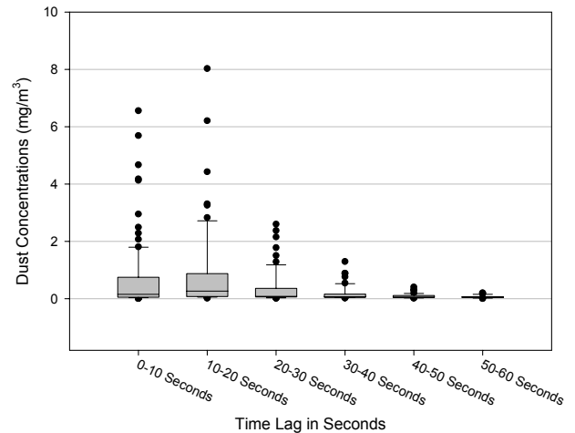
Figure 9. Airborne Respirable Dust Concentrations at Station B for Various Haul Truck Time Lag Intervals from the Stone Quarry Study.
