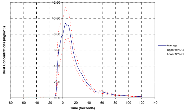
Figure 6. Estimated average instantaneous thoracic dust concentrations for Station A of the Coal Preparation Plant study.
