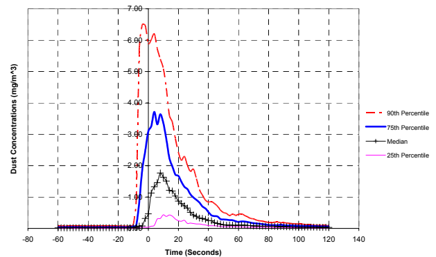
Figure 4. Percentile graph of airborne respirable dust concentrations generated from haul trucks for Station A of the Coal Preparation Plant Study.
