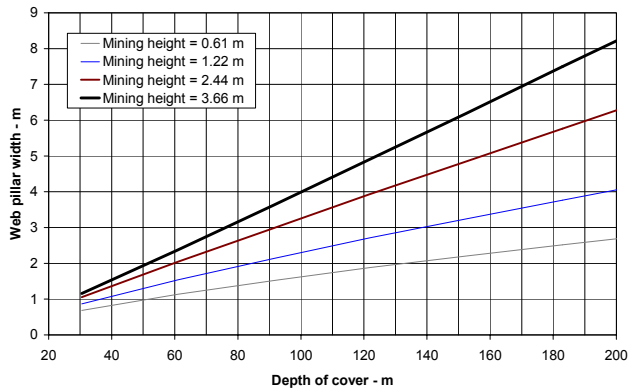
Figure 5B. Suggested web pillar width with stability factor of 1.6, coal strength of 6.2 MPa and 3.66-m-wide hole.
