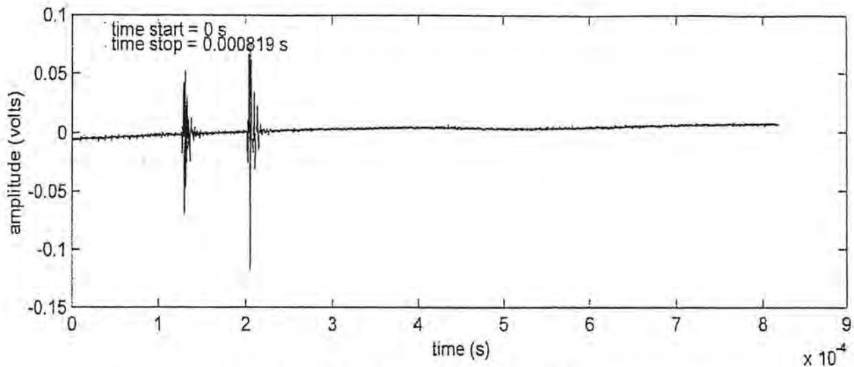
Figure 4.—Air door (electrical noise) waveform.
