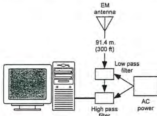
Figure 2.—Schematic of data acquisition system
