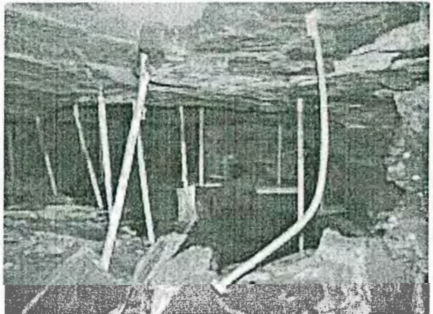
Figure 8. Photograph of roof bolts exposed by weathering of weak shale at Mine B.
