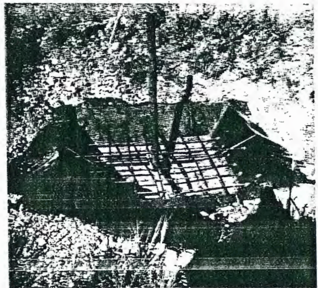
Figure 9.--Ten-ft form showing spider-leg reinforcing over edge of form to support the expanded metal.
