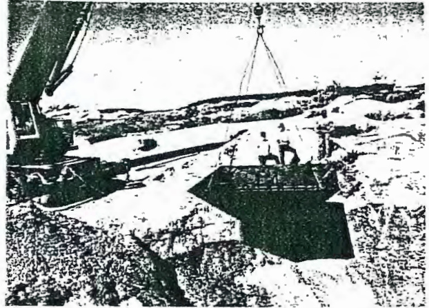
Figure 8.--Lowering 10-ft form into opening.
