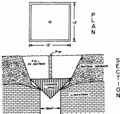
Figure 4.--Installed plug.
