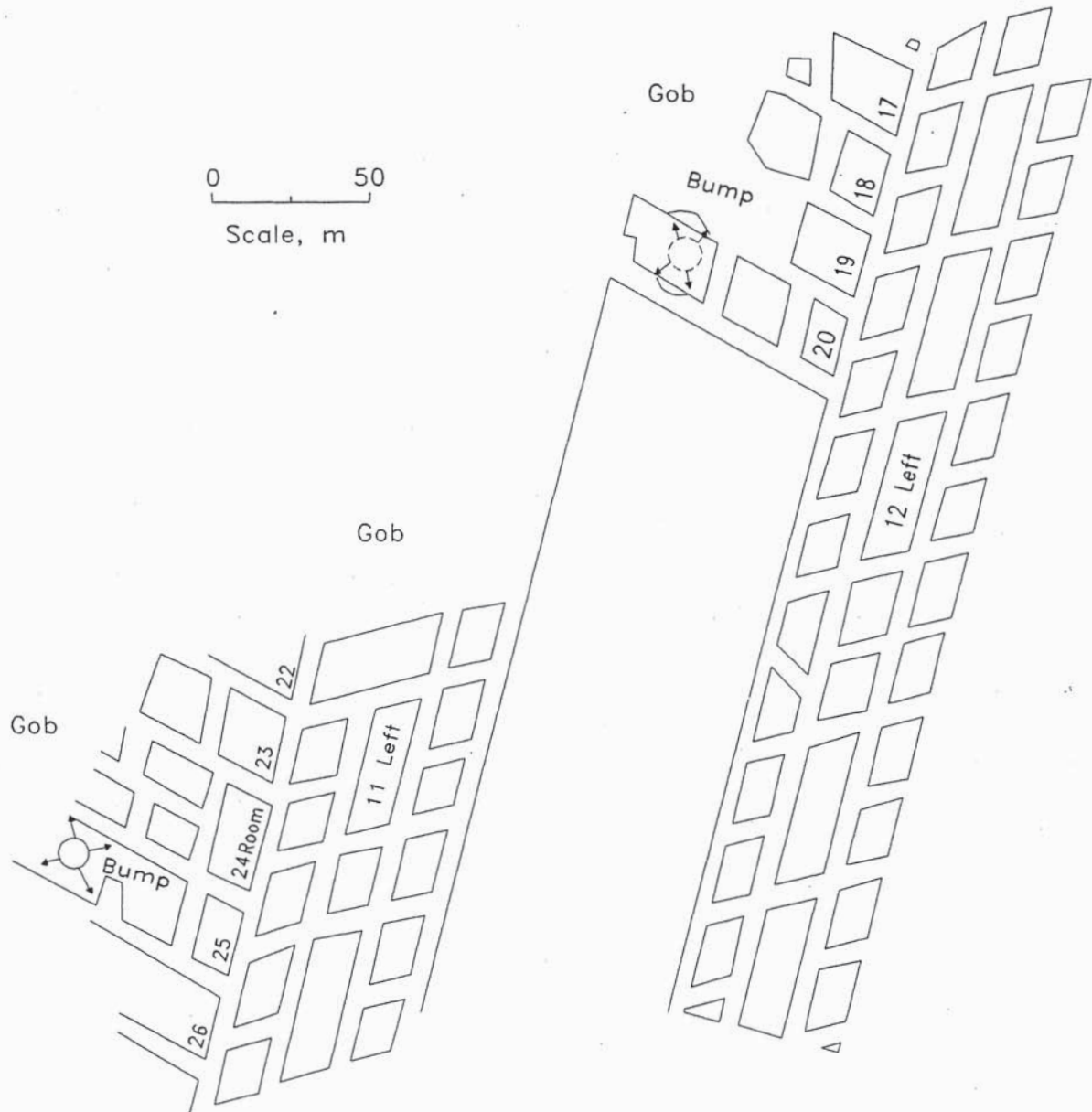
Figure 15 Barrier-Splitting Bumps in Adjacent Sections With Similar Layout Positions, Gary No. 2 Mine, January 1951.
