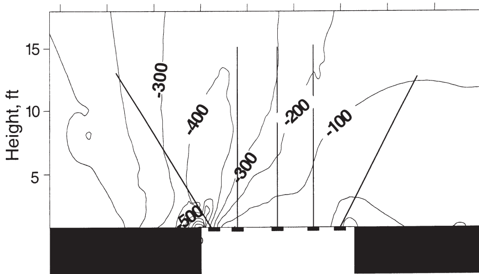
Figure 10. Shear stress distributions across row 1, resin-assisted tensioned bolts, over the recovery room. No cribs installed.
