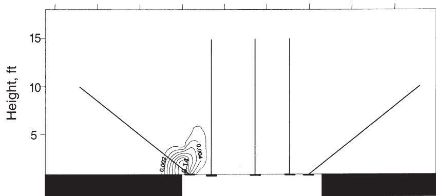
Figure 14. Plastic strain distributions across row 2, cable bolts, over the recovery room. Concrete cribs installed on 10-ft row spacing.
