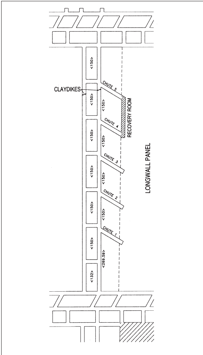
Figure 1. Plan view of longwall recovery area. Recovery room between chutes no. 4 and no. 5.
