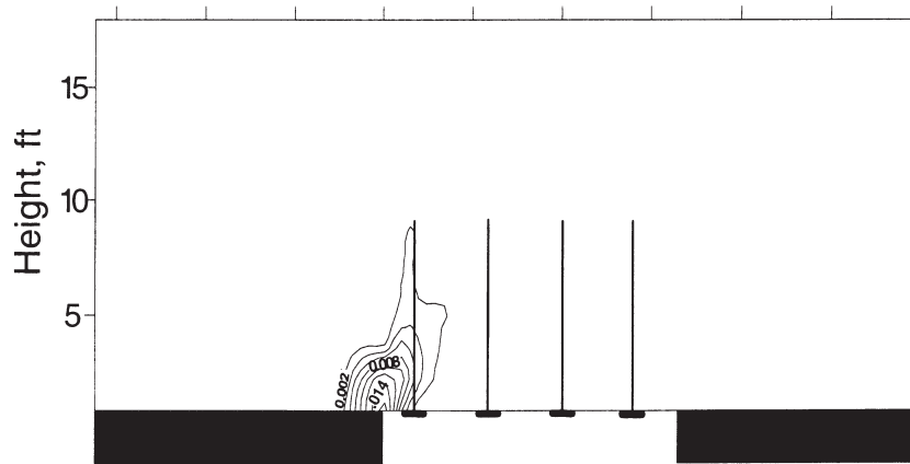
Figure 13. Plastic strain distributions across row 1, resin-assisted tensioned bolts, over the recovery room. Concrete cribs installed on 10-ft row spacing.
