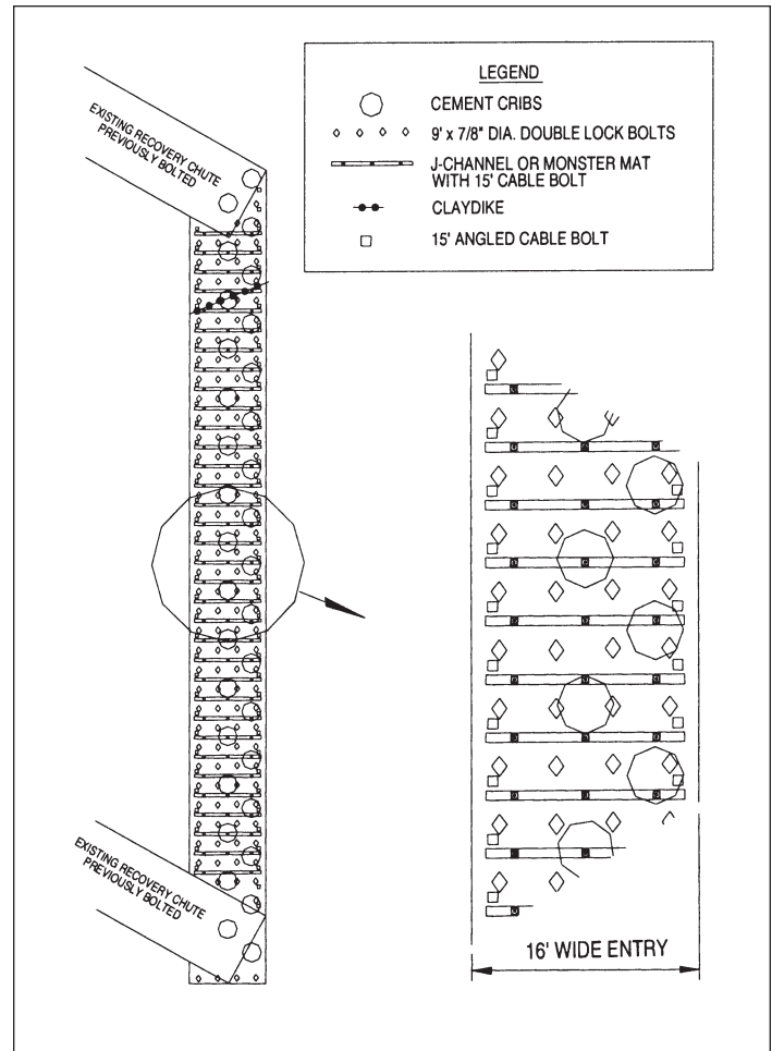
Figure 4. Plan view of the standing support and internal roof reinforcement system.
