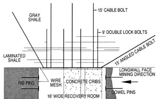
Figure 3. Roof and rib reinforcement system application.
