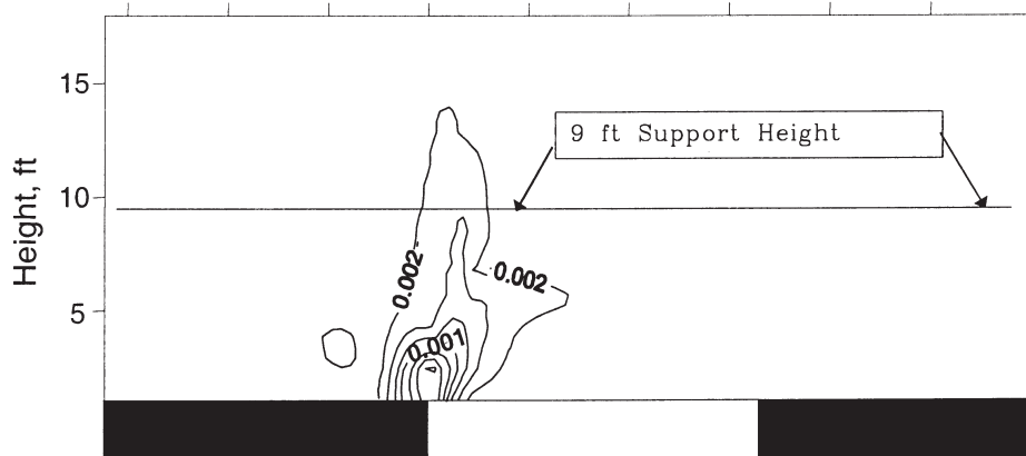
Figure 12. Plastic Strain distributions across row 1, resin-assisted tensioned bolts, over the recovery room. No cribs installed.
