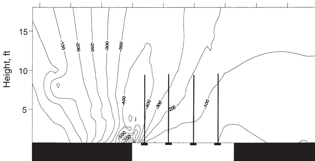
Figure 11. Shear stress distributions across row 2, cable bolts, over the recovery room. No cribs installed.
