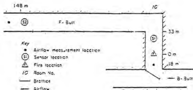
Figure 1. Plan view of mine section.
