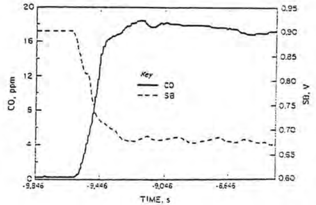
Figure 3. CO and sensor SB response to diesel emissions for experiment No. 4.
