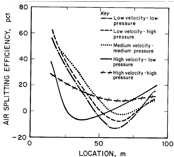
Figure 8. Downstream air-splitting efficiency of air-atomized sprays.
