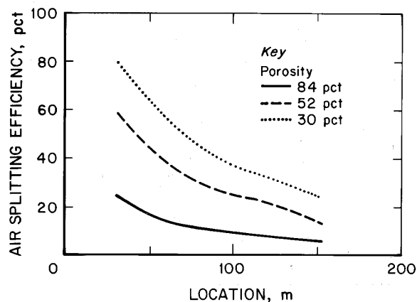
Figure 3. Downstream air-splitting efficiency relationships for the mesh barriers tested.
