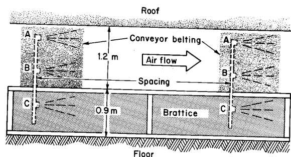
Figure 6. Walkway side view of staged spray layout.
