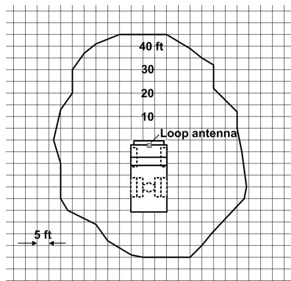
Figure 5. Detection zone for Nautilus Buddy system and person wearing tag.
