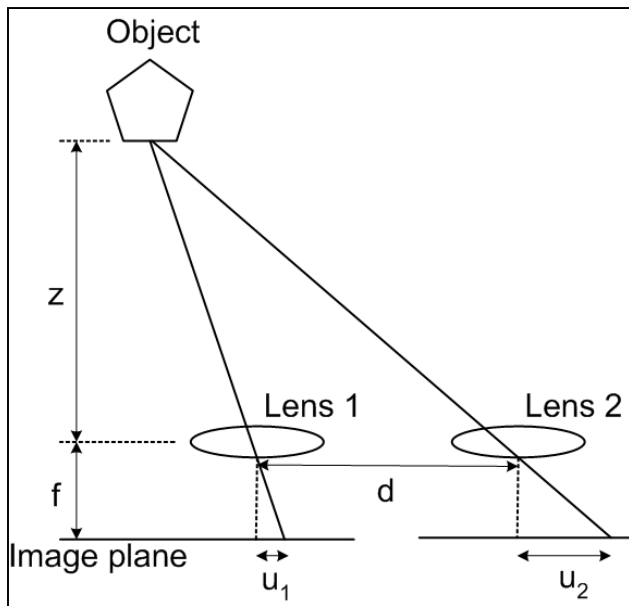
Figure 9. Geometry of stereo imaging and distance calculation.
