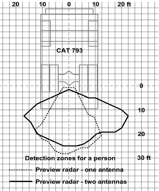
Figure 3. Comparison of detection zones for single- and dual-antenna Preview radar system.
