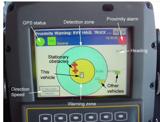
Figure 8. Driver interface for GPS-based proximity warning system.
