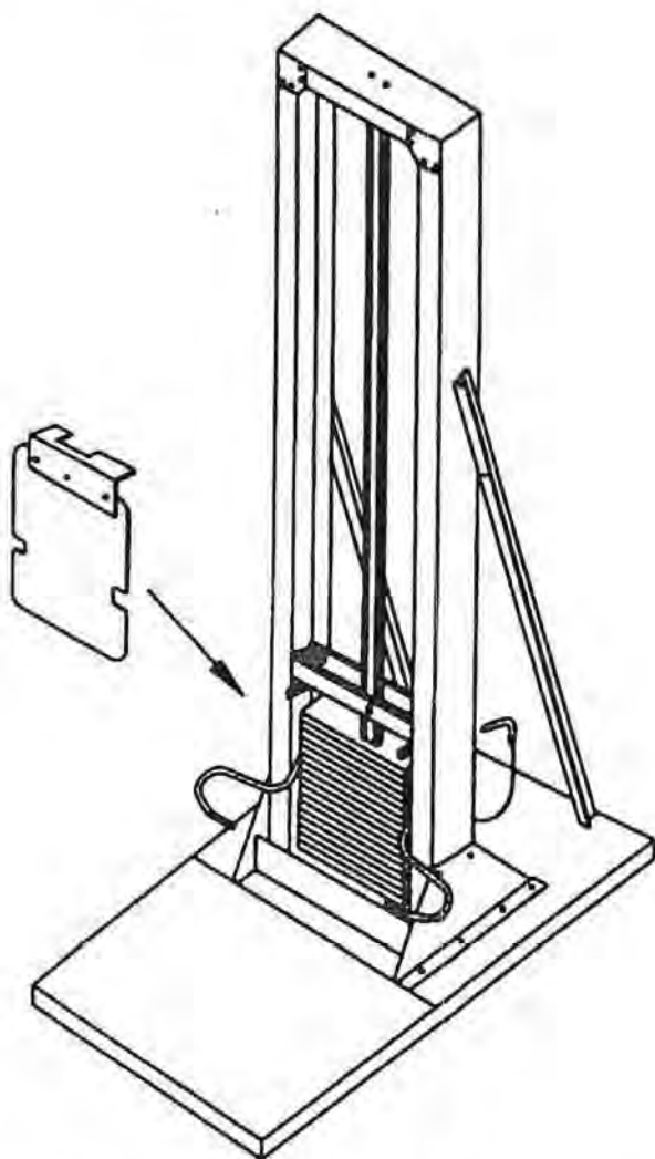
Figure 3. Incremental Weight Lift Machine. The barrier has been removed to expose the hidden stack of weights.
