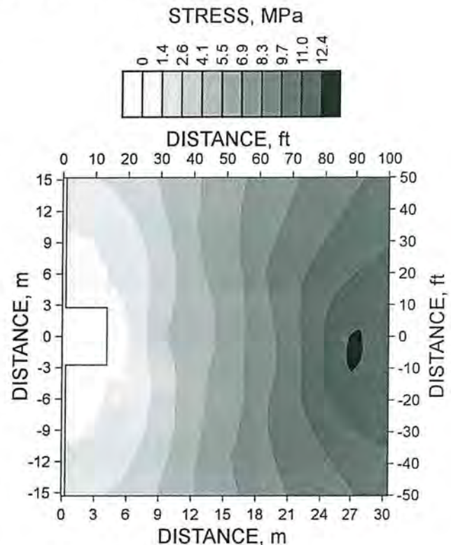
Figure 4. Vertical stress distribution in vicinity of tunnel 25 ft wide by 17 ft high when applied vertical stress equals 1200 psi.
