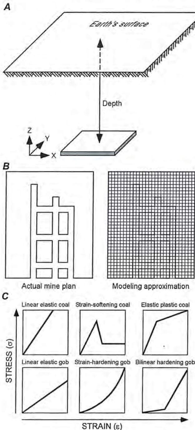
Figure 2. A, Boundary-element seam plane in surrounding rock mass; B, actual mine plan in-seam plane and grid of modeling approximation; C, six different stress-strain models available in Mulsim/NL.
