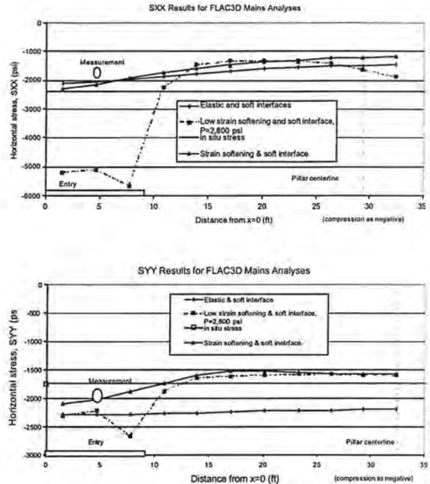
Figure 5. Comparison of the model results versus measured horizontal stresses, Tanoma mine, east mains, 17 ft in roof. Top is Sxx-direction and bottom is Syy-direction.
