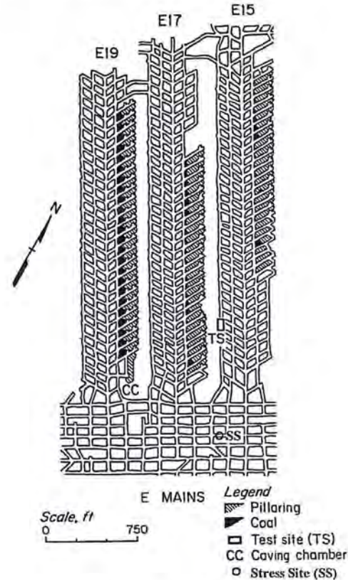
Figure 2. Location of test site (TS) in the L2 entry, stress site (SS).
