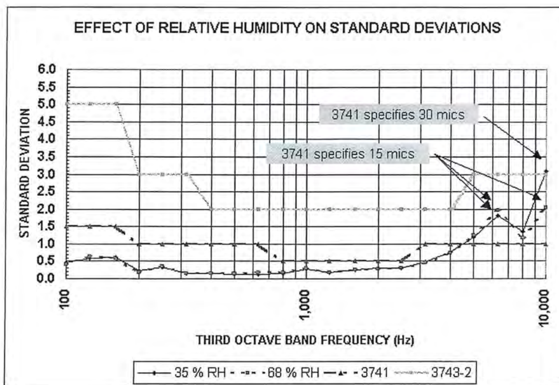
Figure 4. Relative Humidity Effect on Standard Deviations.
