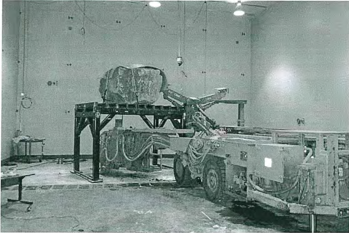
Figure 2. Reverberation Chamber with Roof Bolter During Test Set-up.
