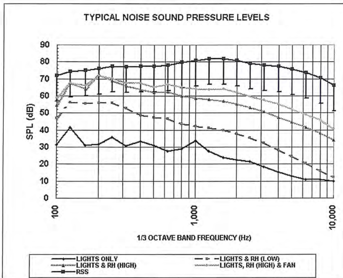
Figure 5. Background Noise Levels.
