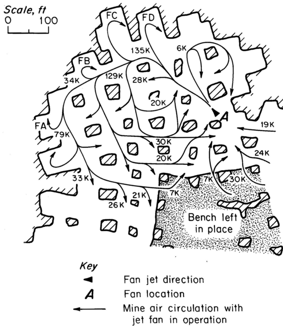
Figure 4-5.—Airflows obtained with jet fan in operation.
