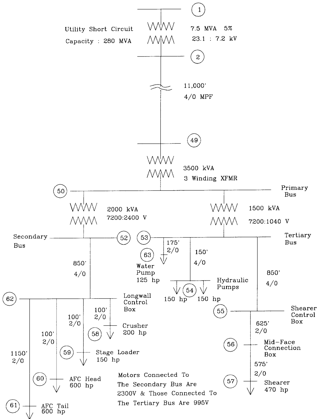
Fig. 3. Example of longwall power system.
