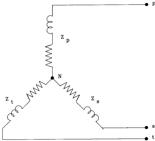
Fig. 1. Single-phase equivalent of three-winding transformer.
